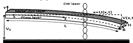
Figure 1: Definition sketch of the laser irradiation initial-boundary-value problem.
