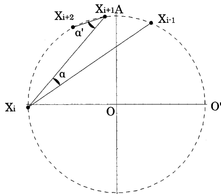
Figure 1: An inner angle which we focus on here is obtained like this figure. In focusing on the consecutive three points, namely X_{i-1} , X_i and X_{i+1} , the objective inner angle in this step is \alpha . The inner angle \alpha' in next step is obtained by the next consecutive points, namely X_i , X_{i+1} and X_{i+2} .
