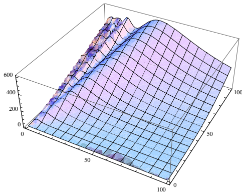
Figure 4: The time-evolution of \tilde{G}_{12} = g(u) after a quantum quench, computed for m = 0.1 and m_0 = 1 using the same approximation in (73). We fixed the phase ambiguity as \theta_0(t) = 0 . The horizontal and vertical coordinate correspond to 1/|k| = \epsilon e^{-u} and t , respectively. The former, 1/|k| , can be interpreted as the z coordinate in the AdS as we explain in section 4. With this interpretation, we can observe, qualitatively, that the excitations induced by the quantum quench are within the light-cone: z < t in the AdS.
