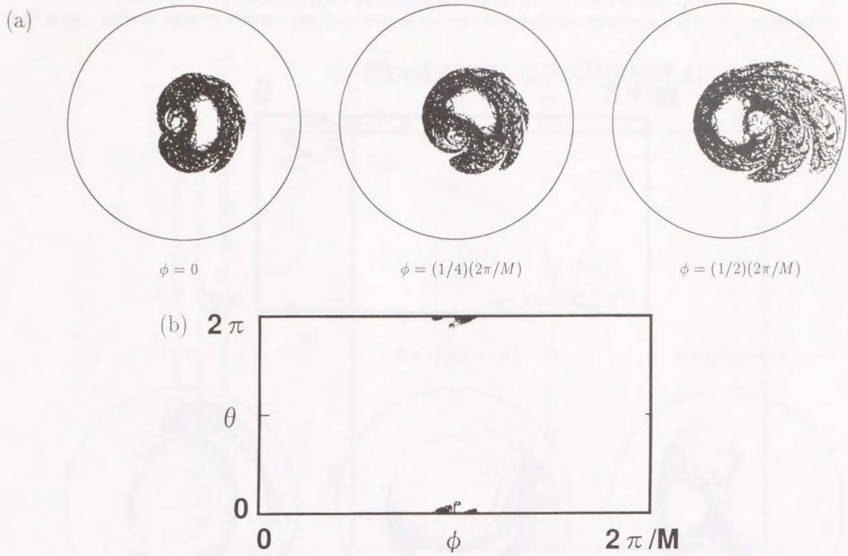
Fig. 3.23: Poincaré plots of magnetic field lines outside the outermost magnetic surface in Heliac-like configuration: (a) traces in \phi = 0 , (1/4)(2\pi/M) and (1/2)(2\pi/M) and (b) traces on the vacuum chamber.
