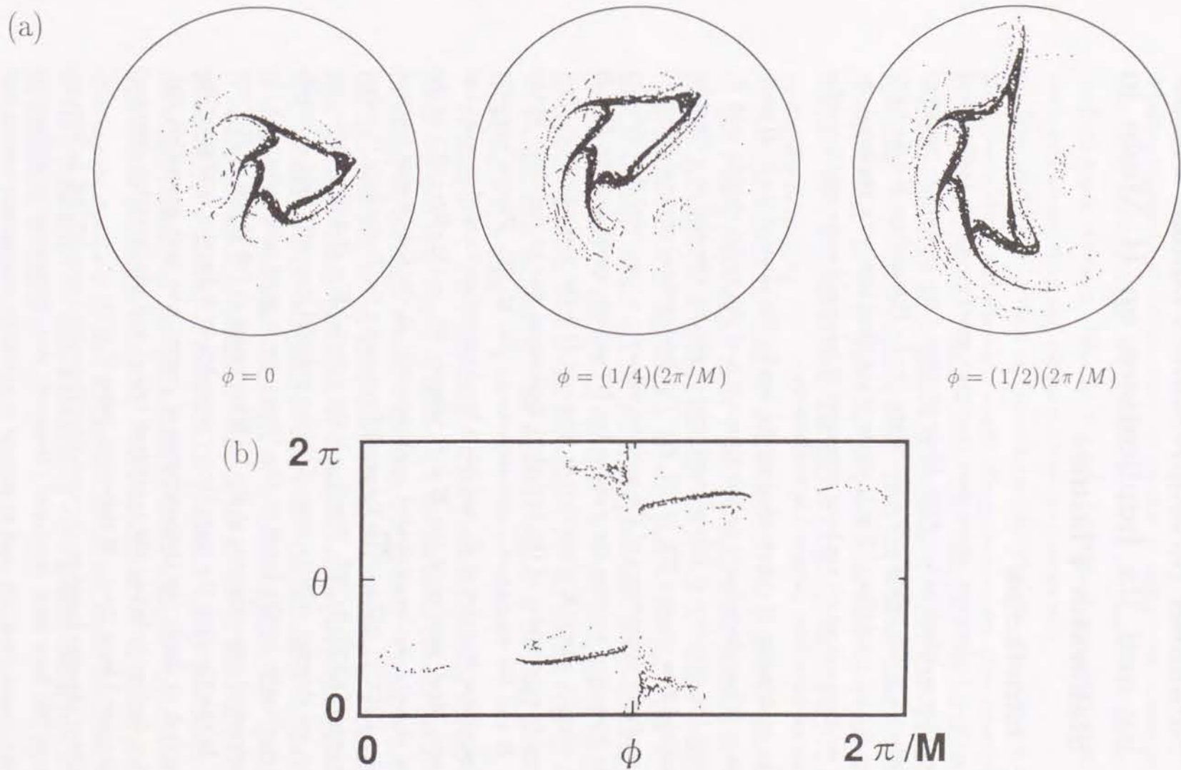
Fig. 3.24: Poincaré plots of magnetic field lines outside the outermost magnetic surface in optimized helical axis configuration: (a) traces in \phi = 0 , (1/4)(2\pi/M) and (1/2)(2\pi/M) and (b) traces on the vacuum chamber.
