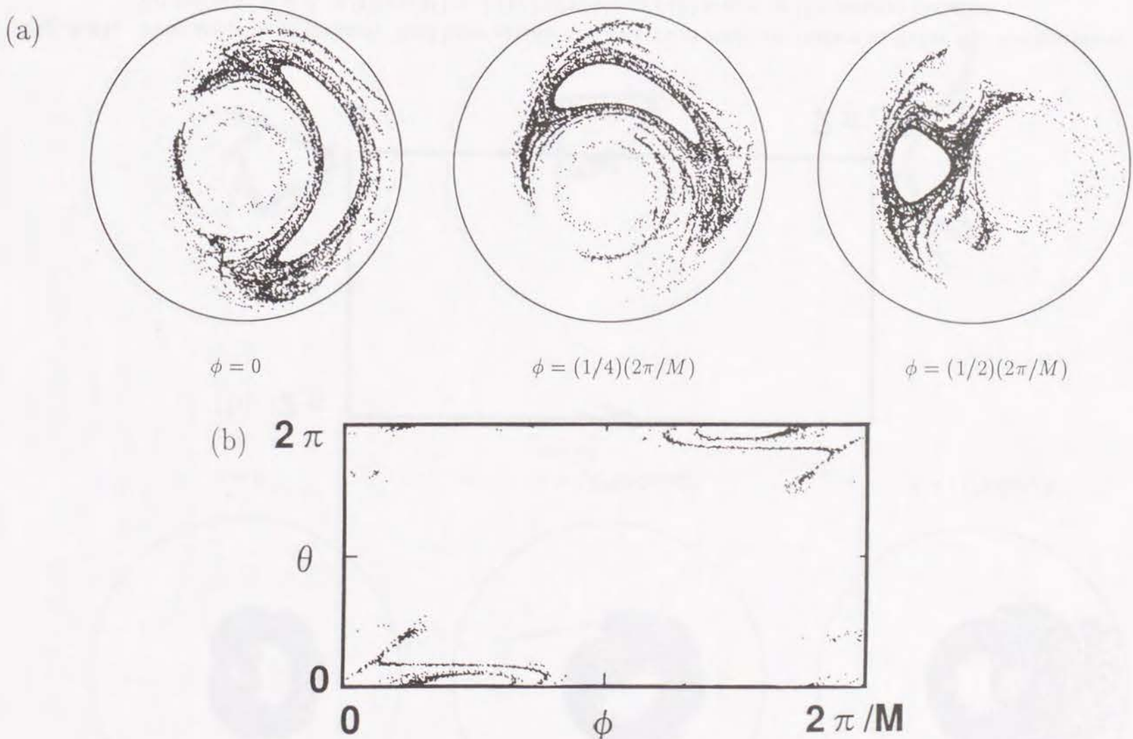
Fig. 3.22: Poincaré plots of magnetic field lines outside the outermost magnetic surface in Helias-like configuration: (a) traces in \phi = 0 , (1/4)(2\pi/M) and (1/2)(2\pi/M) and (b) traces on the vacuum chamber.
