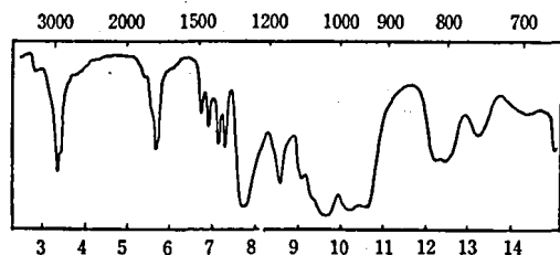
Fig. 1 Infrared Absorption Spectrum of O, O-Diethyl-O-chloroacetyl phosphate (II).
