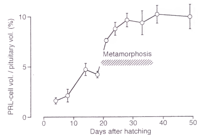
Fig. 3. Developmental changes in the percentage of PRL-cell volume to pituitary volume. Vertical bars represent standard errors of the means of 4 individuals.
