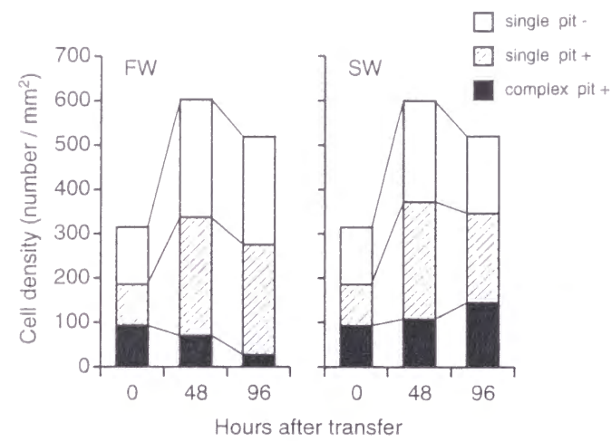
Fig. 7. Time-course changes in the density of three types of \text{Na}^+ , \text{K}^+ -ATPase-immunopositive chloride cells in the yolk-sac membrane of the fish maintained in FW and those transferred to SW. Chloride cells are classified into a single cell without a pit, a single cell with a pit and a multicellular complex with a common pit. Data obtained from four FW and four SW individuals are averaged at each sampling time.
