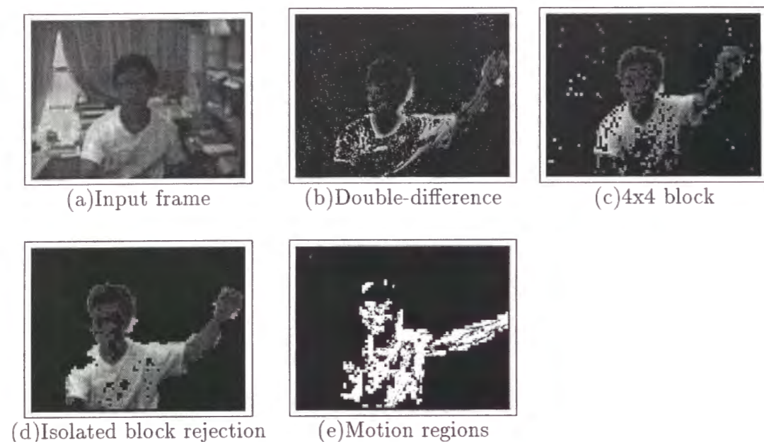
Figure 6.6: Image processing
