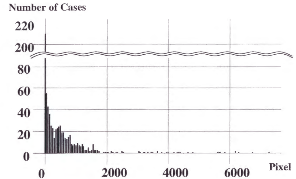
Figure 4.4: Uncovered silhouette area
