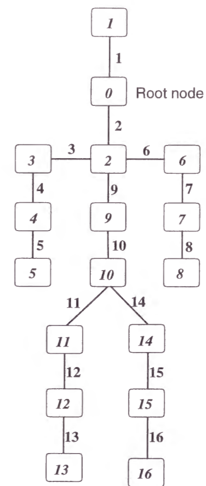
Figure 2.16: PDT of the body model
