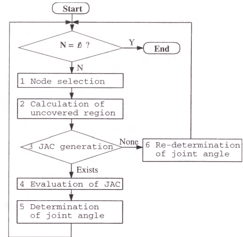
Figure 3.3: Pose estimation procedure
