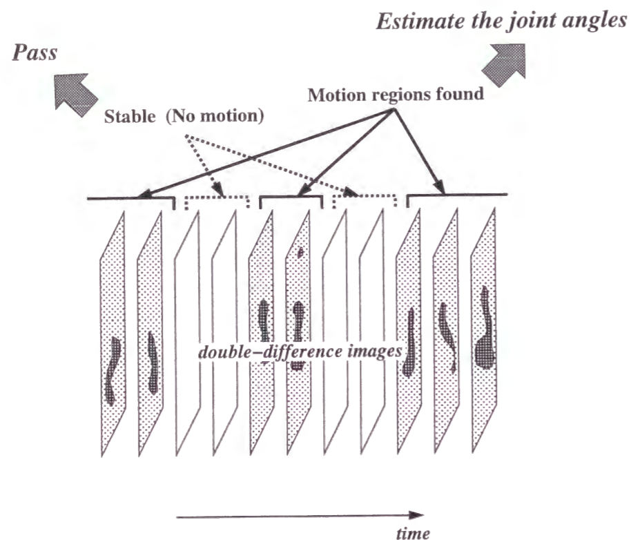
Figure 6.3: Frame skip
