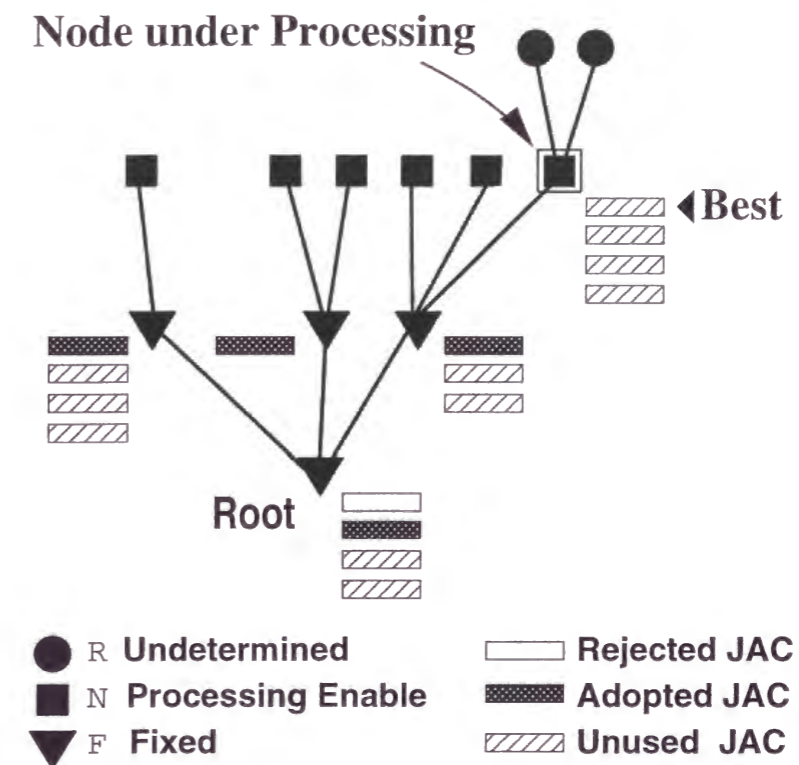
Figure 3.5: A status of a pose decision tree under pose estimation processing
