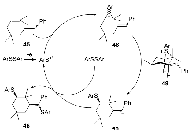
Scheme 16. Mechanism of "ArS + " (=ArS(ArSSAr) + ) initiated addition of ArSSAr to dienes via intramolecular C-C bond formation.
