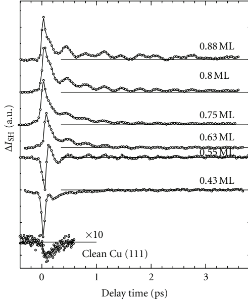
FIGURE 2: Coverage dependence of TRSHG traces for K/Cu(111). Potassium coverages are indicated. 1 ML corresponds to the saturation coverage of the first layer [10]. The pump pulse photon energy was 2.20 eV, and probe pulse photon energy was 1.55 eV.
