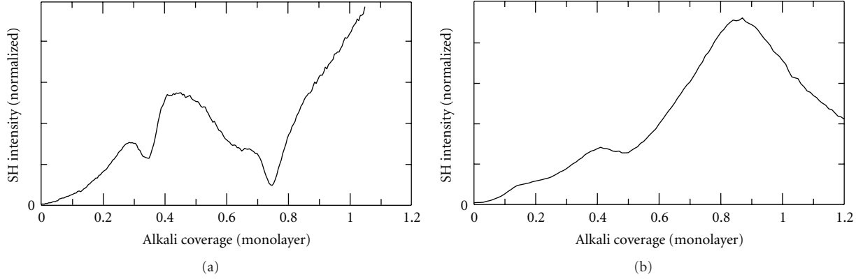
FIGURE 1: Second harmonic intensity as a function of coverage of (a) potassium and (b) cesium on Cu(111) surface. The excitation wavelength is 800 nm (1.55 eV). Note that here one monolayer corresponds to the saturation coverage of the first layer, although in the original papers one monolayer has been defined as the atomic densities of the substrates.
