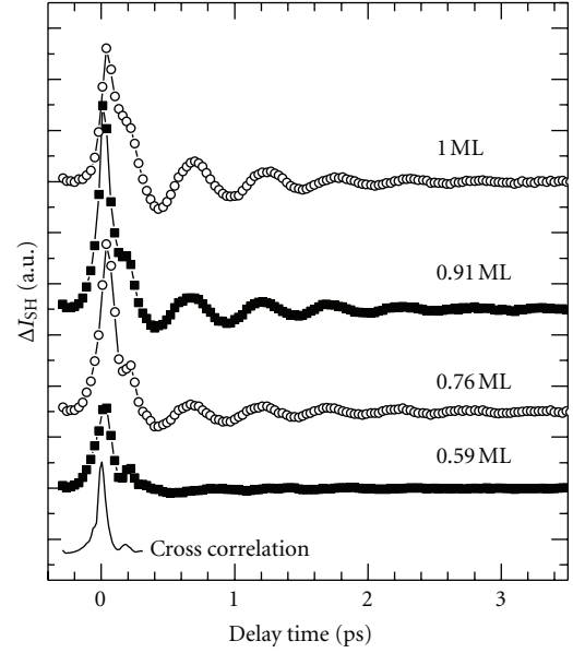
FIGURE 3: Coverage dependence of TRSHG traces for Cs/Cu(111). Cesium coverages are indicated. 1 ML corresponds to the saturation coverage of the first layer. The bottom trace is a cross-correlation curve between pump and probe. The pump pulse photon energy was 1.55 eV, while the probe pulse photon energy was 2.20 eV.
