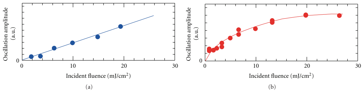
FIGURE 6: Incident pump fluence dependence of the initial amplitude of oscillation in TRSHG traces from Cs-covered Cu(111). The excitation wavelengths were (a) \lambda_{\text{ex}} = 400 nm (blue) and (b) \lambda_{\text{ex}} = 800 nm (red). Solid lines are guides to the eye. Reprinted with permission from [11]. Copyright (2011) American Chemical Society.
