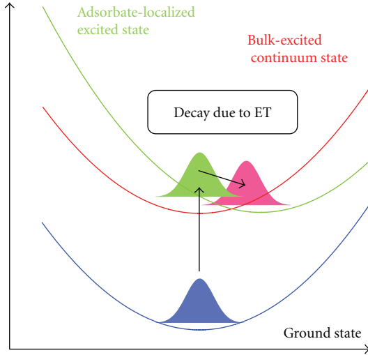
FIGURE 7: Schematic representation of the potential energy curves (PECs) of the TAM model: ground state (blue), the adsorbate-localized excited state (green), and the bulk continuum states (red). Reprinted with permission from [11]. Copyright (2011) American Chemical Society.
