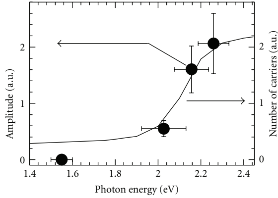
FIGURE 4: Excitation photon energy dependence of the initial amplitude of the coherent vibration of the S mode of K/Cu(111) (filled circles). The potassium coverage was 0.63 ML. Numerical estimation of the number of photogenerated carriers within the Cu substrate [10] (solid curve).
