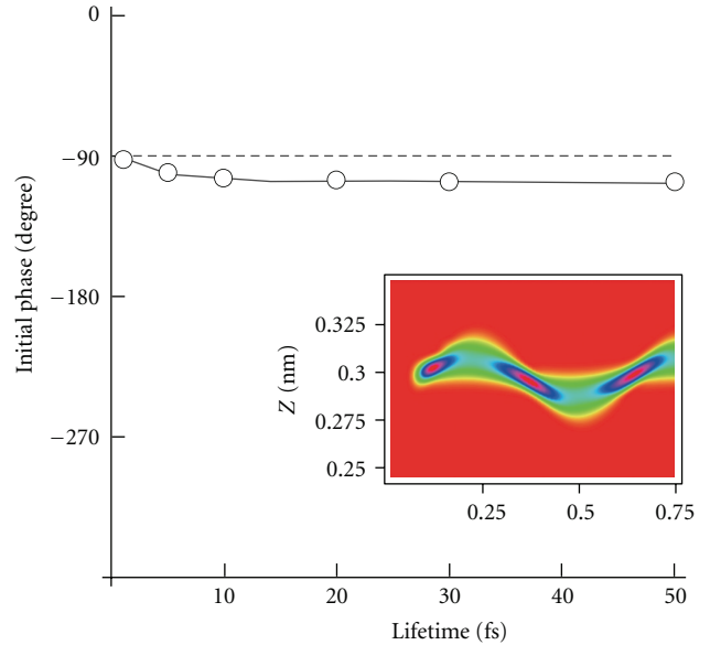
FIGURE 8: Initial phases calculated from TAM model as a function of the lifetime of the excited state. Inset: the time evolution of the wave packet. Reprinted with permission from [11]. Copyright (2011) American Chemical Society.
