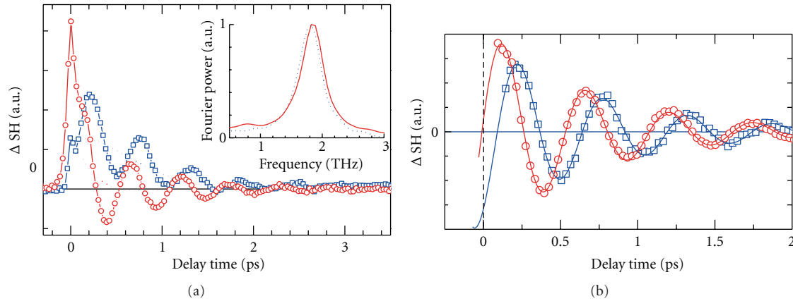
FIGURE 5: (a) TRSHG traces for Cs/Cu(111) with \lambda_{\text{ex}} = 800 nm (1.55 eV) (red) and 400 nm (3.10 eV) (blue). The probe wavelength was 565 nm (2.20 eV). Cs coverage was 0.8 ML for \lambda_{\text{ex}} = 800 nm and 0.9 ML for \lambda_{\text{ex}} = 400 nm. The inset shows the Fourier spectra of the oscillatory components. (b) The oscillatory parts of the TRSHG traces in (a). Reprinted with permission from [11]. Copyright (2011) American Chemical Society.
