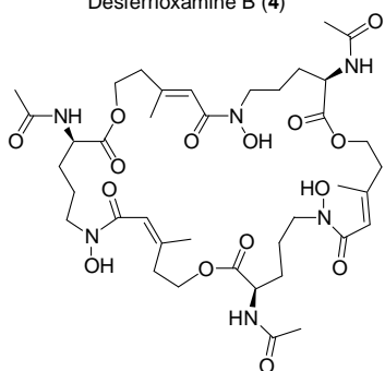
Desferritriacetylfulsarine C (5)
