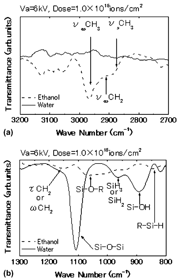
FIG. 15. Transmittance of the Si(100) surfaces irradiated by ethanol and water cluster ions for the wave numbers of (a) 2700–3200 cm -1 and (b) 800–1300 cm -1 , respectively.
