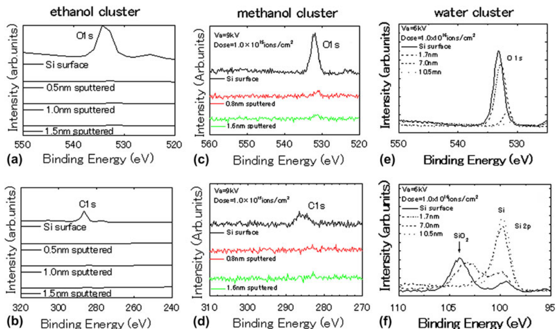
FIG. 7. Depth profile of the x-ray photoelectron spectroscopy peaks for the Si surfaces irradiated by (a, b) ethanol cluster ions, (c, d) methanol cluster ions, and (e, f) water cluster ions.
