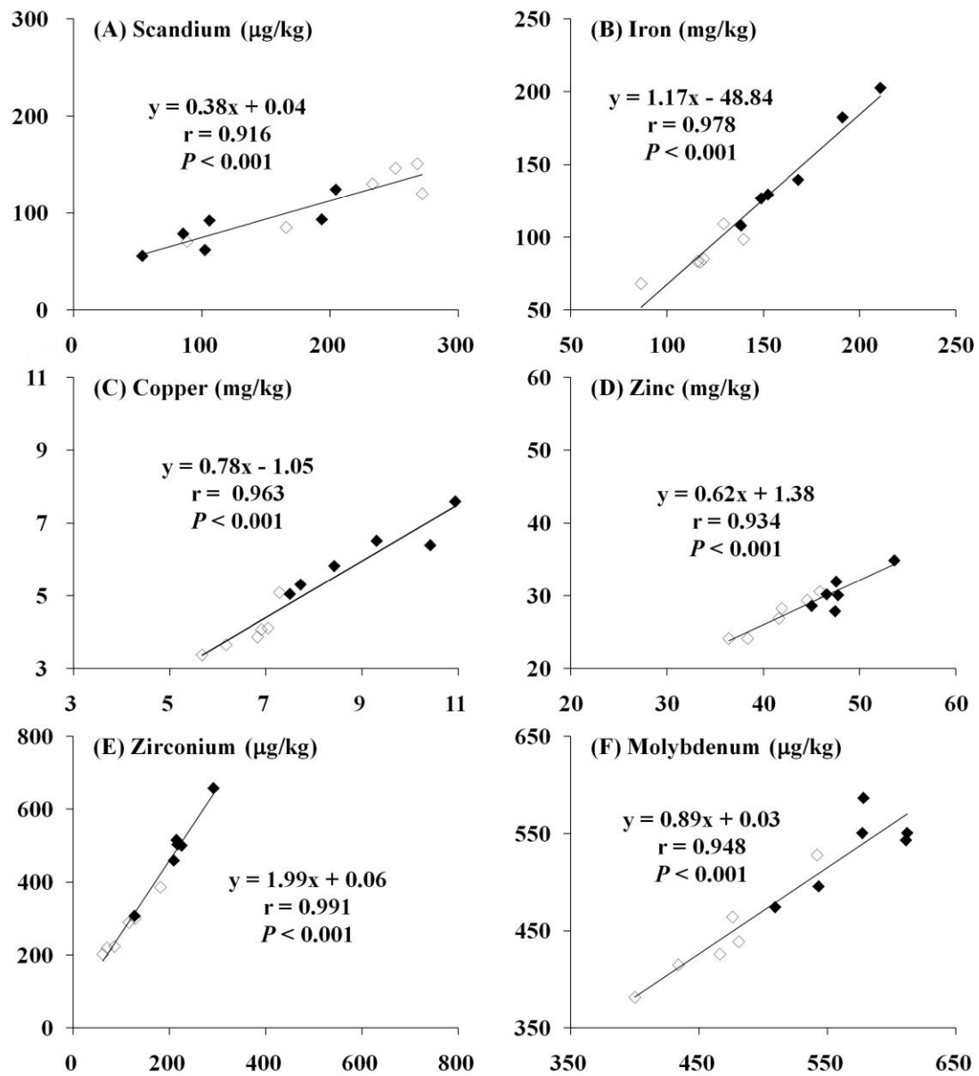
Figure 1. Correlations between semiquantitative measurements and quantitative measurements of some trace minerals. (◇) and (◆) showed control and magnesium deficient rats, respectively. The x- and y-axis showed the concentration determined by the semiquantitative analysis and the quantitative analyses, respectively. P values are significant level of correlations between semiquantitative measurements and quantitative measurements.
