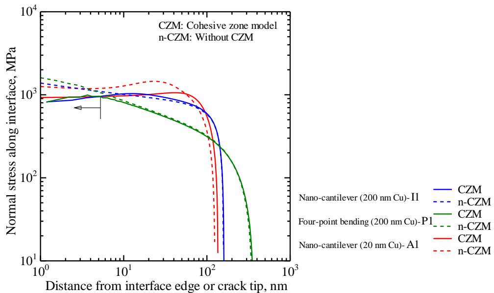
Fig. 11 Comparison of the stress distributions along the Cu/Si interface of different specimens with and without CZM
