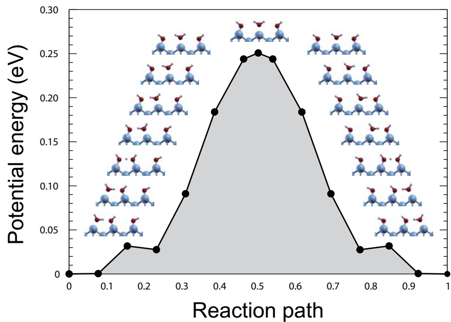
FIG. 4. Calculated potential energy surface for the H-atom relay reaction in an \text{H}_2\text{O}-(\text{OH})_2 chain along the [001] direction. The set of images from initial to final states, shown as insets, were determined by the nudged elastic band method (see Supplementary Information). The H-transfer to the center OH is facile ( \lesssim 0.04 eV). The transition state (0.25 eV) corresponds to \text{OH}-\text{H}_2\text{O}-\text{OH} with a broken H bond.
