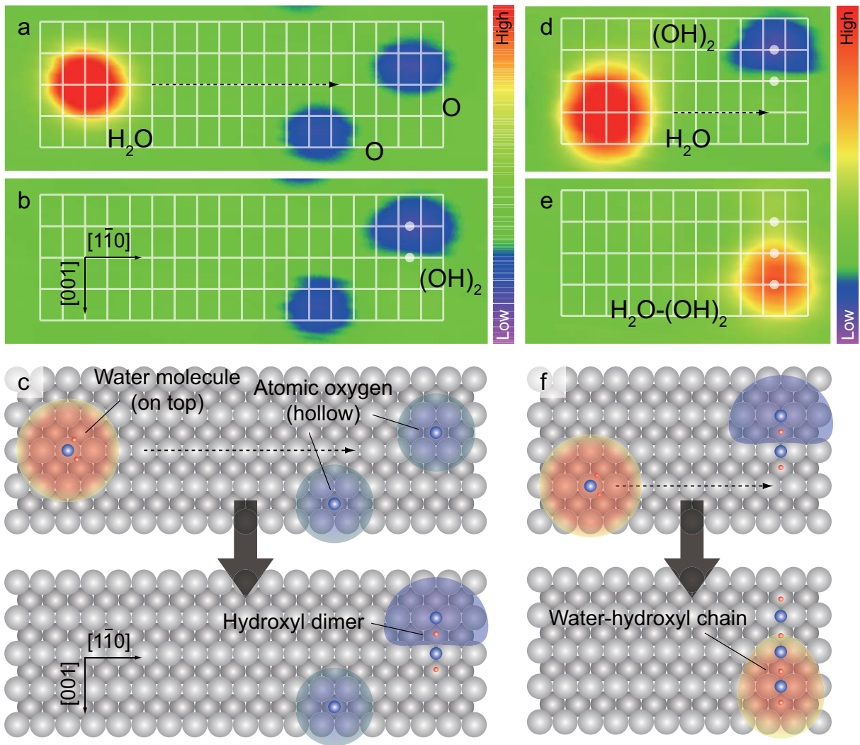
FIG. 1. Sequential STM images of the assembly process of the \text{H}_2\text{O}-(\text{OH})_2 chain from individual water molecules on Cu(110). The images were recorded in constant current mode at a sample bias voltage of V=24 mV and tunneling current of I=0.5 nA. (a) A water molecule and two atomic oxygen are imaged as a round protrusion and two depressions, respectively. The white grid lines indicate the lattice of Cu(110). The water molecule was dragged along the [1\bar{1}0] direction toward atomic oxygen (dashed arrow). (b) The reactants yield an OH dimer imaged as a semicircular depression. The white dots indicate the short-bridge sites to which oxygen atoms in (\text{OH})_2 are bonded. (c) Schematic illustration of the reaction process. The light gray circles represent Cu atoms on the substrate which form “Cu rows” along the [1\bar{1}0] direction. STM images of water, oxygen atoms and (\text{OH})_2 are also depicted. (d), (e) Subsequently, another water molecule was dragged to the end of (\text{OH})_2 (dashed arrow), then yielding an \text{H}_2\text{O}-(\text{OH})_2 complex in a chain form. The three dots in (e) depict the nearest short-bridge sites to which oxygen atoms in the complex are bonded. It is noted that the positions of oxygen atoms deviate slightly from the exact short-bridge sites along [001] axis, as shown in the structure optimized by DFT calculations [Fig. 2(a) and (b)]. (f) Schematic illustration of the reaction process of (d) and (e). The image sizes are 20 \times 58 \text{ \AA}^2 for (a) and (b), and 20 \times 36 \text{ \AA}^2 for (d) and (e).
