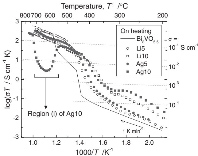
Fig. 4 Reprinted data of changes in electrical conductivity of \text{Bi}_2\text{VO}_{5.5} , Li5, Li10, Ag5, and Ag10. 8) Pellets with Au electrodes were quenched from 800^\circ\text{C} ( \text{Bi}_2\text{VO}_{5.5} ), 700^\circ\text{C} (Li5, Li10, and Ag5), or 750^\circ\text{C} (Ag10) just before measurements. Samples were heated at 1 \text{ K min}^{-1} under flowing artificial air. A distinct conductivity change was observed in region (i) for Ag10.
