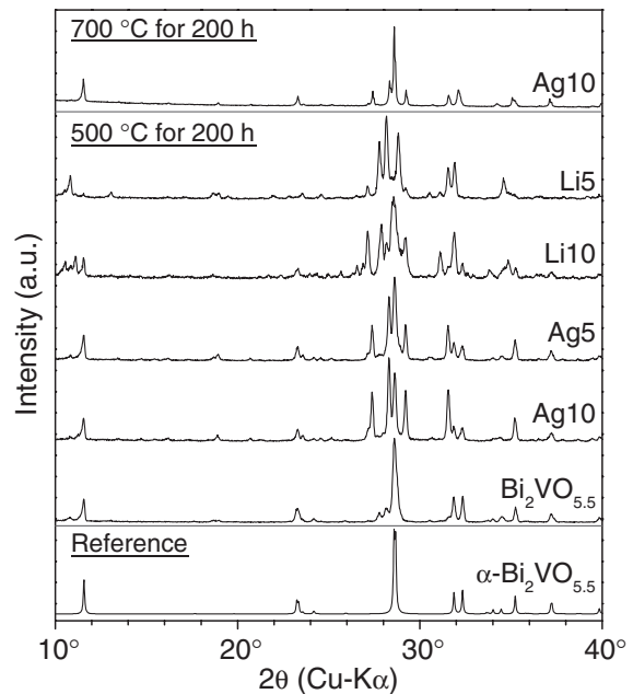
Fig. 6 XRD patterns of powders after annealing at 500 or 700^\circ\text{C} for 200 h. The calculated pattern of \alpha\text{-Bi}_2\text{VO}_{5.5} is shown for reference. 7) The composition of the secondary phase in Ag10 annealed at 700^\circ\text{C} is determined to be \text{Bi}_{14}\text{V}_5\text{AgO}_{34} by EDX.
