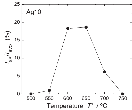
Fig. 5 Variation in the amount of secondary phase in Ag10. I_{\text{SP}} / I_{\text{BVO}} , which is the ratio of the relative intensity of the maximum peak of the secondary phase at \sim 27.1^\circ shown in Fig. 3(d) to the maximum peak of the BIMEVOX phase, is plotted as a function of temperature.
