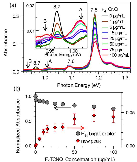
FIG. 2 (color online). (a) The hole-doping dependence of the absorption spectra of CoMoCAT-PFO nanotubes. The inset shows an enlarged view of the lower-energy region where the new peaks appear. The new peaks indicated by the arrows A and B are associated with (7,5) and (7,6) nanotubes, respectively. (b) The hole-doping dependence of the absorption intensity of the E_{11} bright excitons (left axis) and the new peak (right axis) of (7,5) carbon nanotubes.
