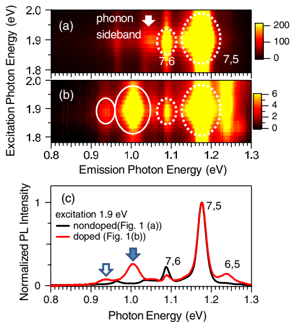
FIG. 1 (color online). PLE contour maps of (a) nondoped CoMoCAT-PFO nanotubes, (b) CoMoCAT-PFO nanotubes doped with F_4TCNQ solutions (200 \mu\text{g}/\text{mL} ). The dotted circles show the E_{11} bright excitons and the solid circles show the new PL peaks due to hole doping. (c) The normalized PL spectra of the nondoped and doped CoMoCAT-PFO nanotubes [from (a) and (b), respectively] at the excitation photon energy of 1.9 eV. The doping-induced new PL peaks of (7,5) and (7,6) nanotubes are indicated by the solid and open arrows, respectively.
