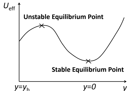
FIG. 1. Effective potential in the KR model.
