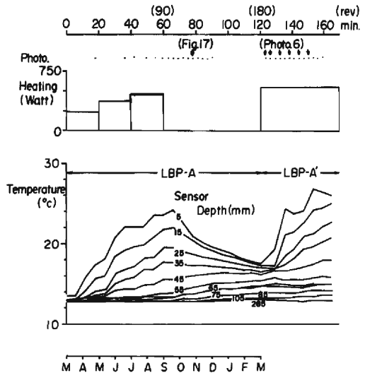
Fig. 16 Experimental conditions and temperature records of LBP-A and LBP-A'. The thermo-couples depths are 5, 15, 25, 35, 45, 55, 65, 75, 85 mm (10 mm interval) and 105, 135, 165, 195, 225, 255, 285 mm (30 mm interval).
