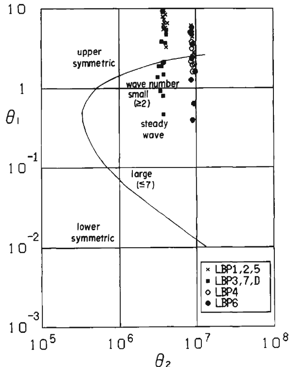
Fig. 32 Regime diagram
