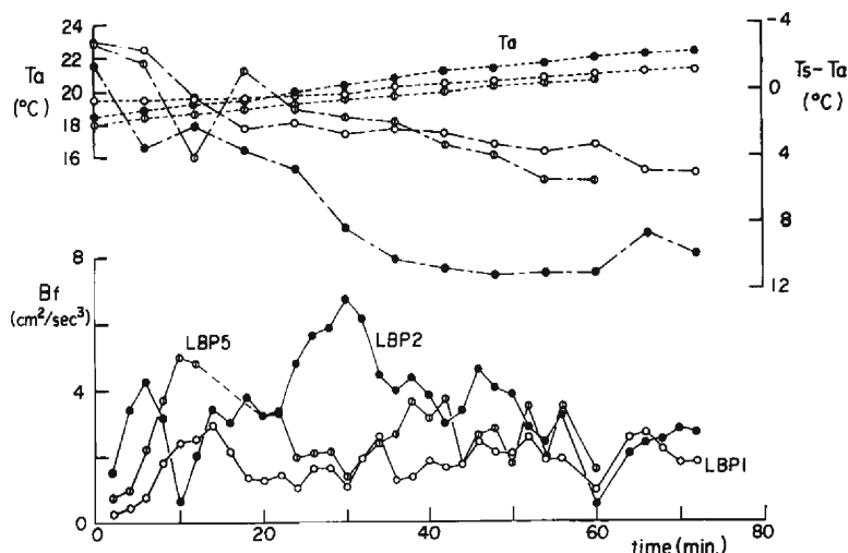
Fig. 26 The buoyancy flux estimated as the time change of the upper layer buoyancy, air temperature and its difference with the surface temperature (as D1) in LBP1, 2 and 5
