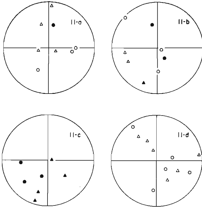
Fig. 20. The directional distribution of subsequent earthquakes. ○, △; T \leq 20000 min and L \leq 40 km (in 11-a and b), T \leq 10000 min and L \leq 30 km (in 11-d), ●, ▲; T = 7354 min and L = 5.4 km (in 11-a), T \leq 1000 min and L \leq 20 km (in 11-b and c).
