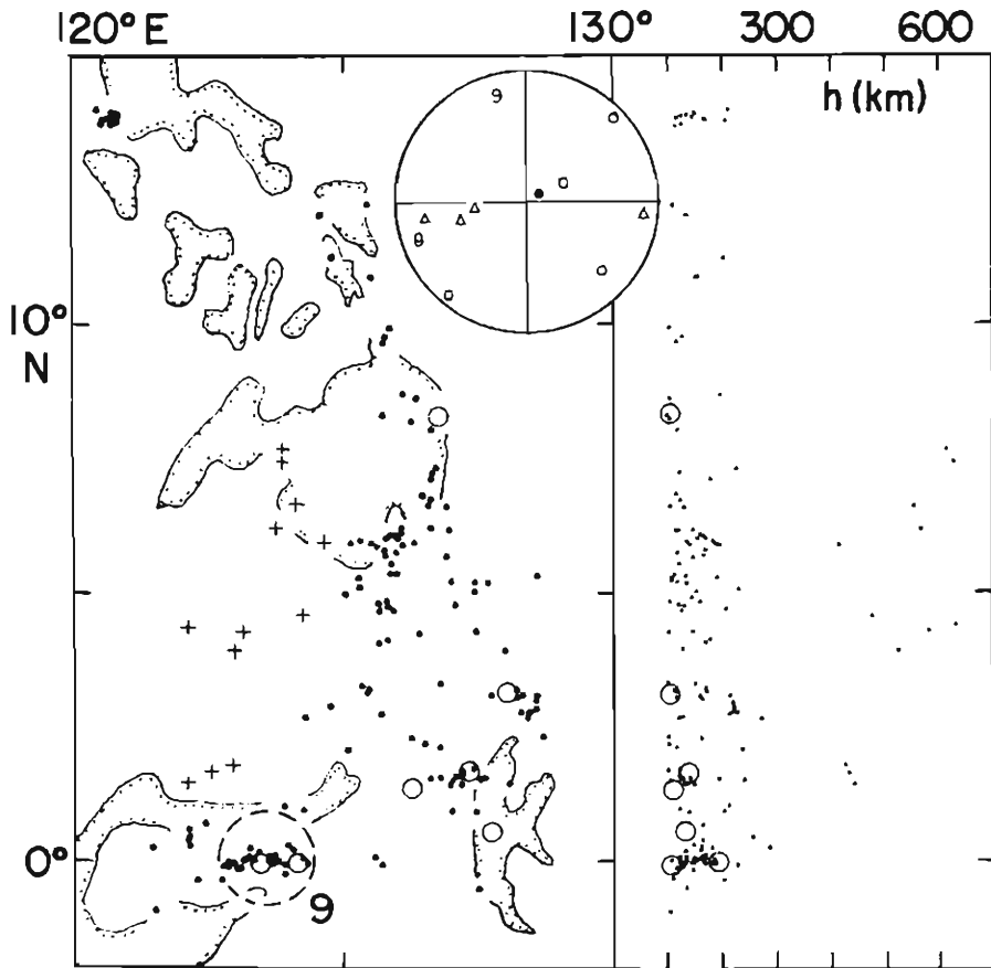
Fig. 15. Philippines-Celebes region.
