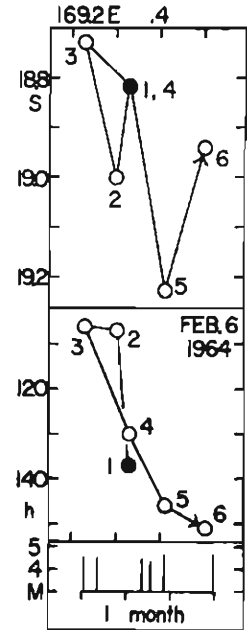
Fig. 21. A multiplet near the 11-d area.
