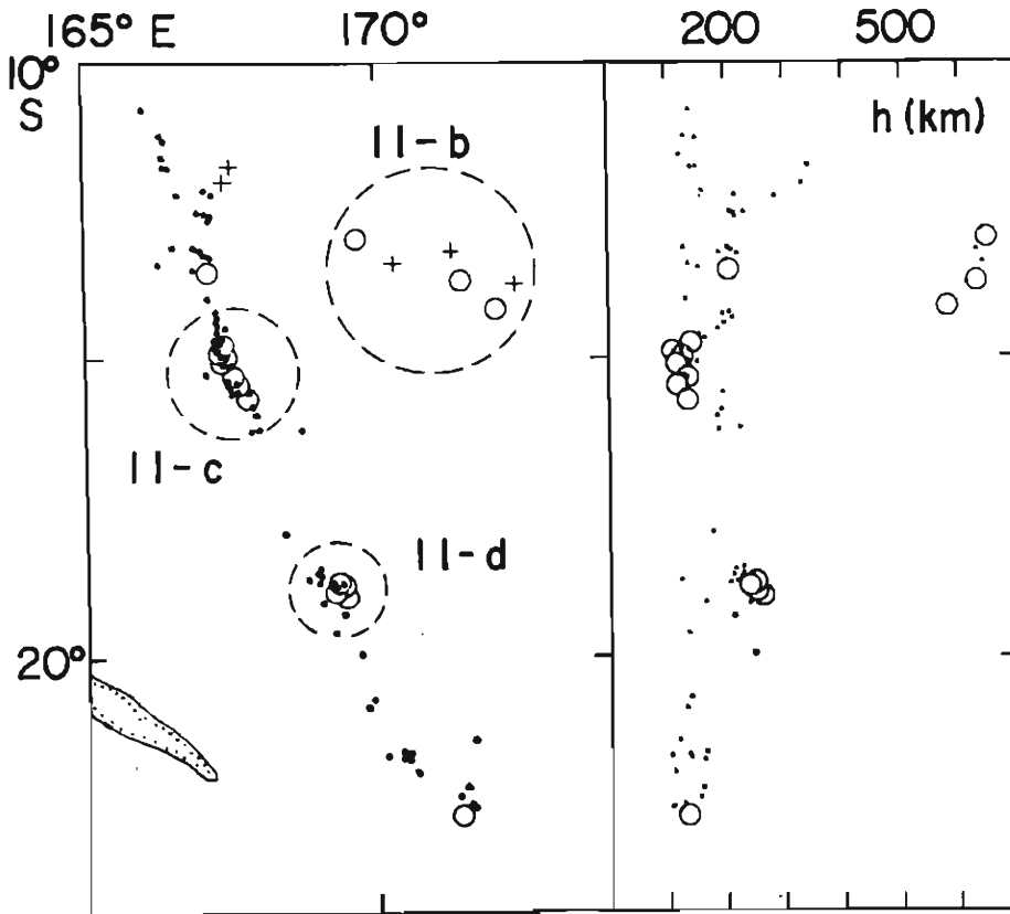
Fig. 19. New Hebrides region.
