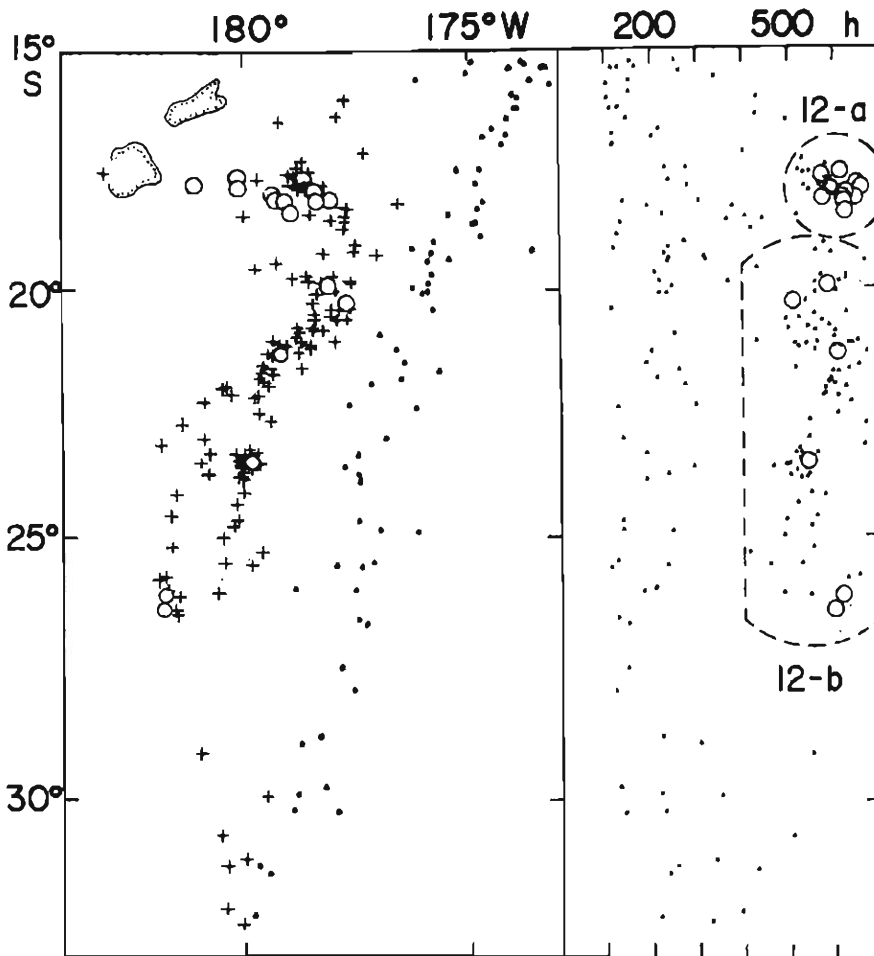
Fig. 22. Fiji-Tonga-Kermadec region.
