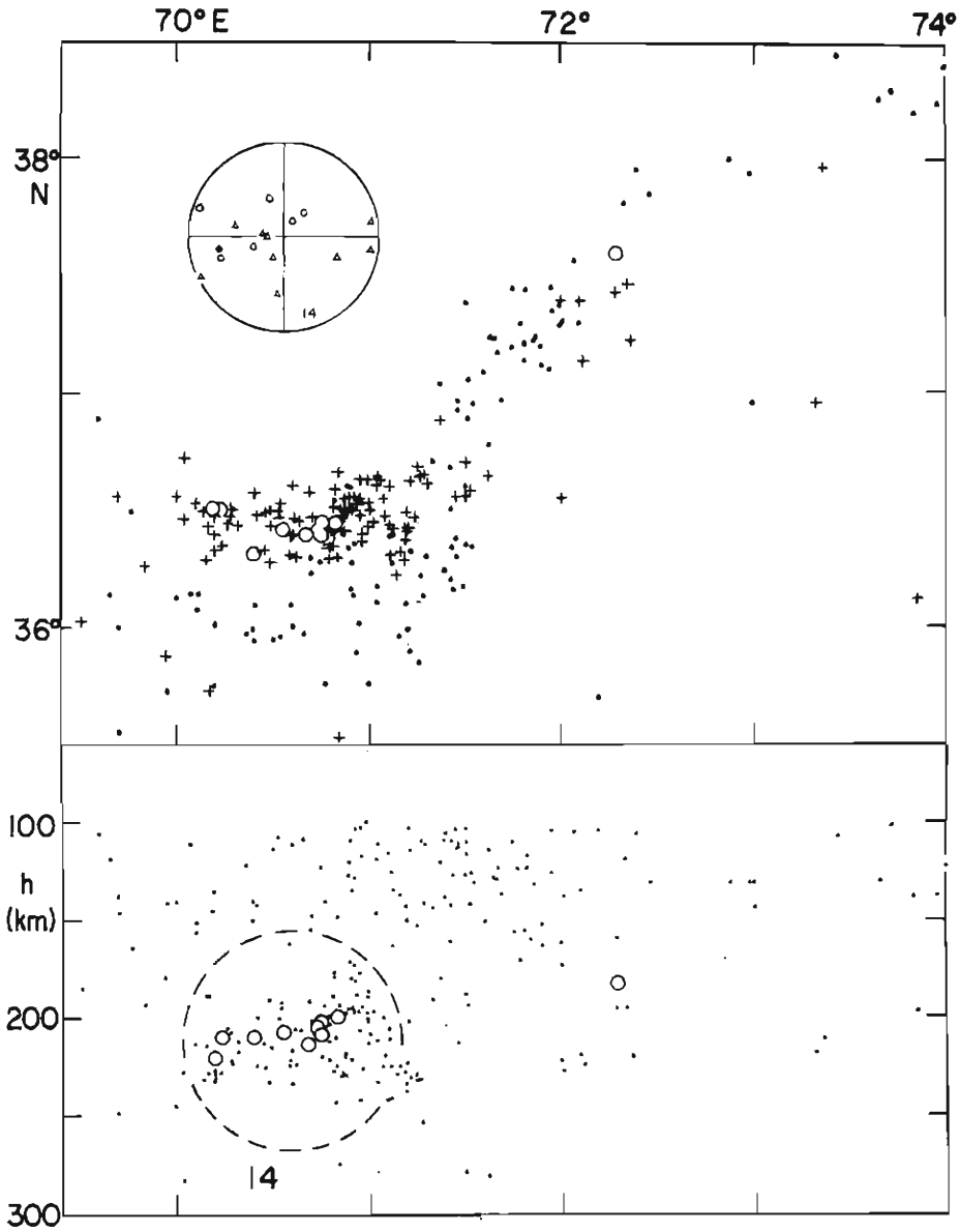
Fig. 26. Hindu-Kush region. · ; h = 100-179 km, + ; h = 180-300 km, ○ ; Multiplets of T \leq 5000 min and L \leq 20 km. In the directional distribution, ○, △ ; T \leq 5000 min and L \leq 20 km, ● ; T = 357 min and L = 20.3 km.
