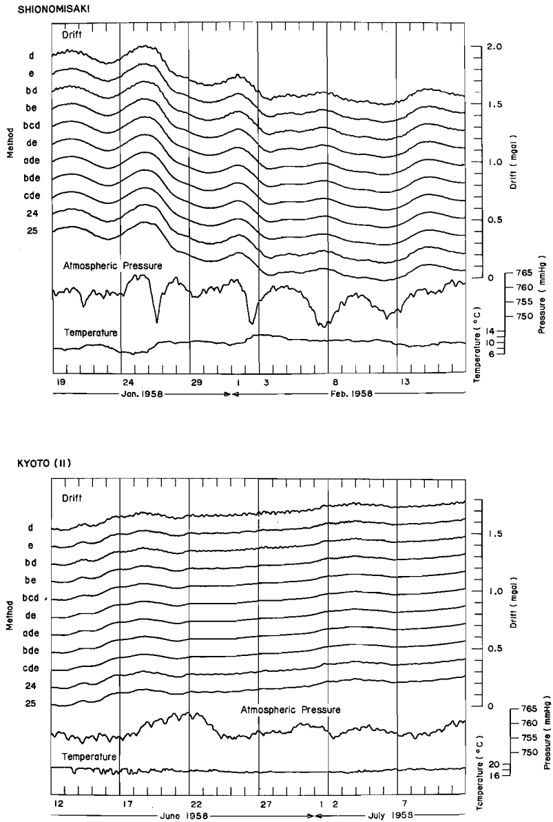
Fig. 2.4. Drift curves obtained by the various methods from the data observed at two stations—Shionomisaki (upper figure) and Kyoto (II) —and the changes of atmospheric pressure and room temperature.
