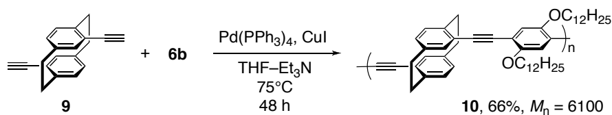
Scheme 3. Synthesis of polymer 10 containing pseudo- para -linked [2.2]paracyclophane
