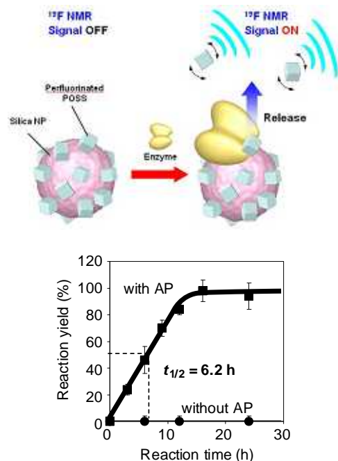
Fig. 1 Time-course of the enzymatic reaction. F-POSS-coated silica NPs (1.5 mg) were incubated in 500 \mu L of the reaction solutions containing AP (5 U) (square dots) and non-containing AP (circular dots) in 50 mM sodium phosphate, 25 mM Tris-HCl, and 0.05 mM EDTA (pH = 7.0) at 37 ^{\circ} C. The reaction yields were monitored with ^{19} F NMR and calculated by the fitting on the standard curve.
