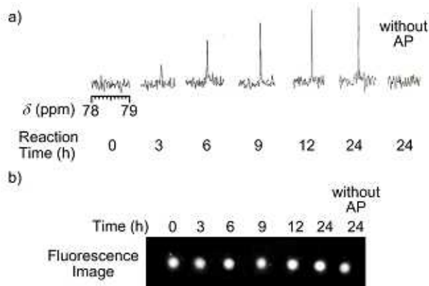
Fig. 2 (a) ^{19} F NMR spectra of F-POSS-coated silica NPs in diameter of 150 nm containing fluorescein-5(6)-carboxylic acid in enzymatic hydrolysis with AP. (b) The fluorescence image was taken using a transilluminator (365 nm) through a 480-nm long pass emission filter.
