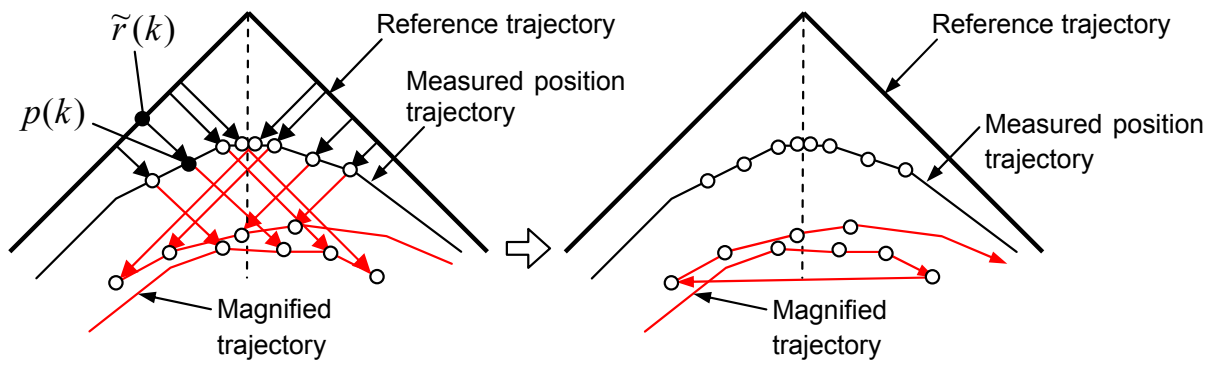
Fig. 2. Schematics of the conventional magnification of contouring error at a square corner.
