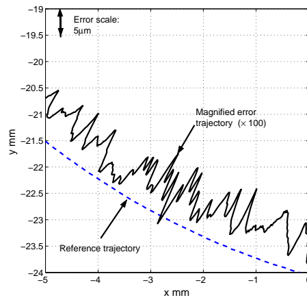
(d) Proposed magnification (the area indicated in (c) is zoomed in).
