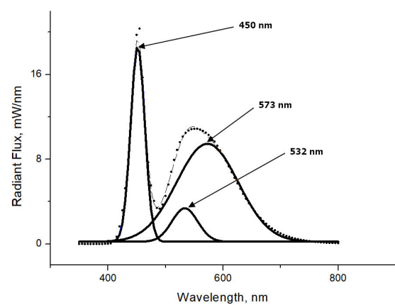
Fig. 4. Result of approximation of the white LED spectra by three Gaussian curves
