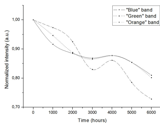
Fig. 5. Intensity variation of separate bands during 6000 h aging: a – quasi-absolute; b – normalized
