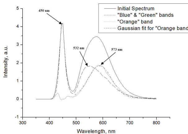
Fig. 3. Result of the Alentsev-Fok method application for deconvolution of the white LED spectra
