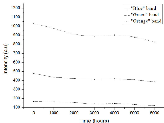
Fig. 5. Intensity variation of separate bands during 6000 h aging: a – quasi-absolute; b – normalized
