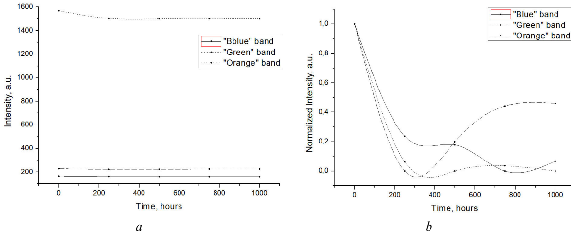
Fig. 6. Intensity variation of separate bands during 1000 h aging at 50 °C temperature: a – quasi-absolute; b – normalized
