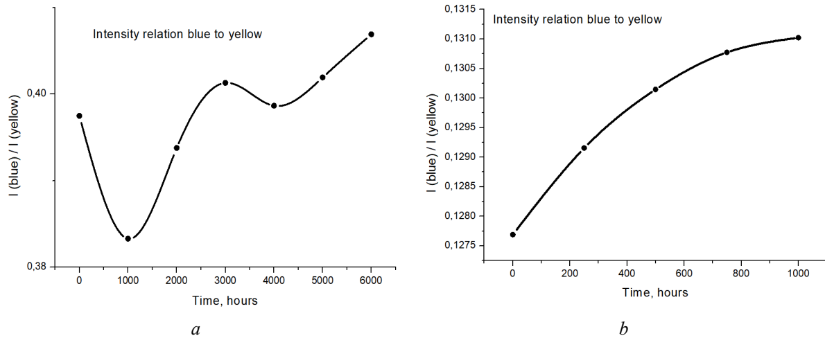
Fig.7 Intensity variation of “blue” to “yellow” bands relation: a – during 6000 h aging; b – during 1000 h aging at 50 °C temperature
