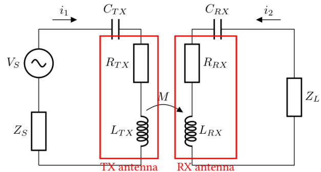
Figure 5: Inductive coupling between reader and transponder.
