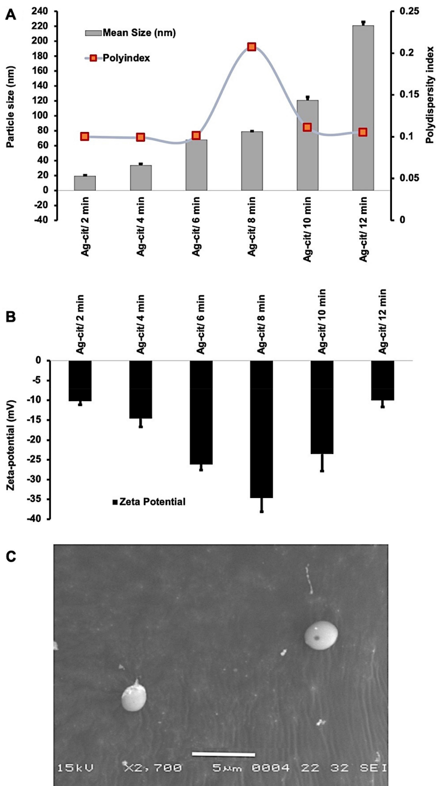
Figure 2 The size distribution of AgNPs-CIT; (A). The mean particle size (nm), (B). ζ-potentials (mV), and polydispersity indices of all AgNPs-CIT at 2, 4, 6, 8, 10, and 12 min; (C). SEM image of AgNPs-CIT reduced after 10 min.
