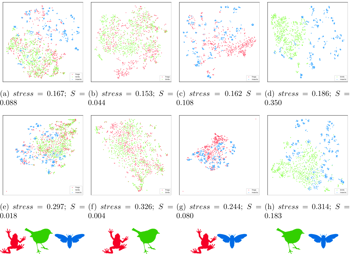
Fig. 6. Visualization of data sets: columns from left to right show results for DS1, DS2, DS3 and DS4. In the 1st row (a-d) t-SNE projections are shown for the data sets with 30, 30, 46 and 41 best features respectively. 2nd row (e-h) shows t-SNE projections for the same data sets employing the complete set of 238 features.
