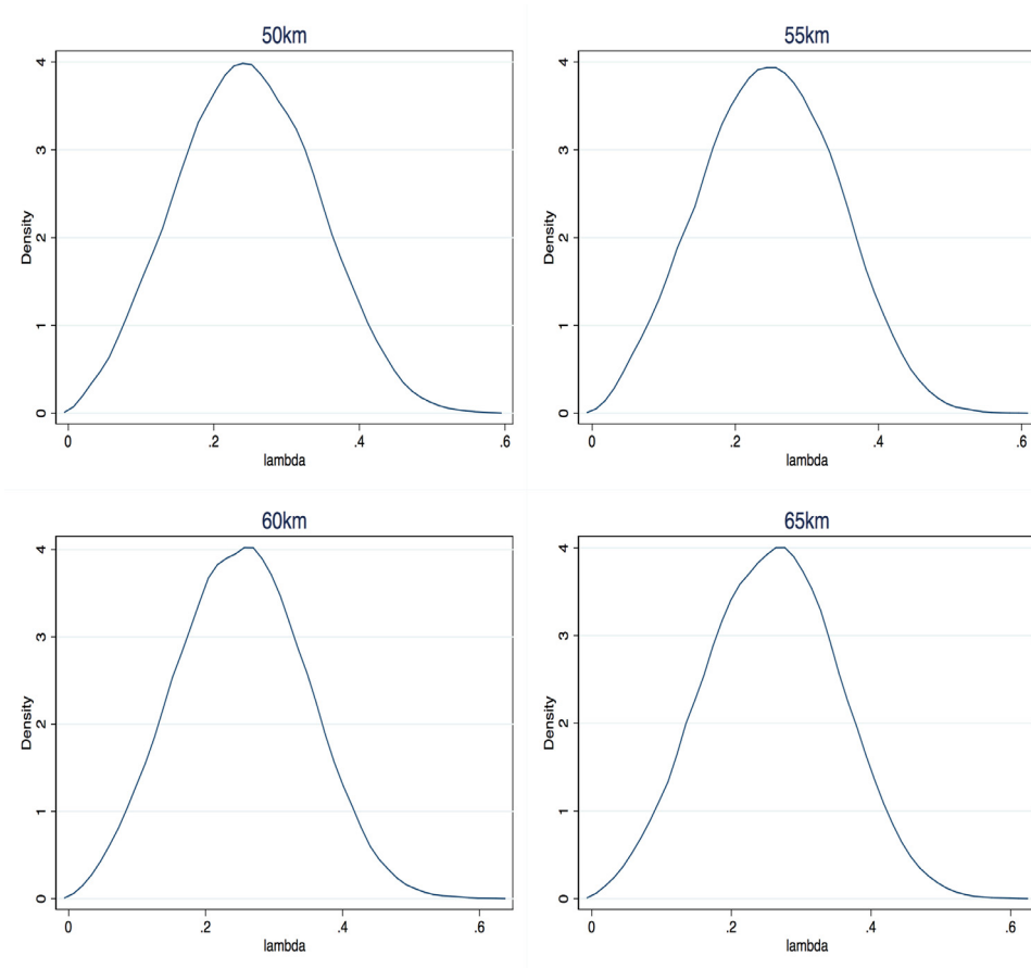
Fig. A2. Posterior distributions of \lambda for the different cut-off points.
