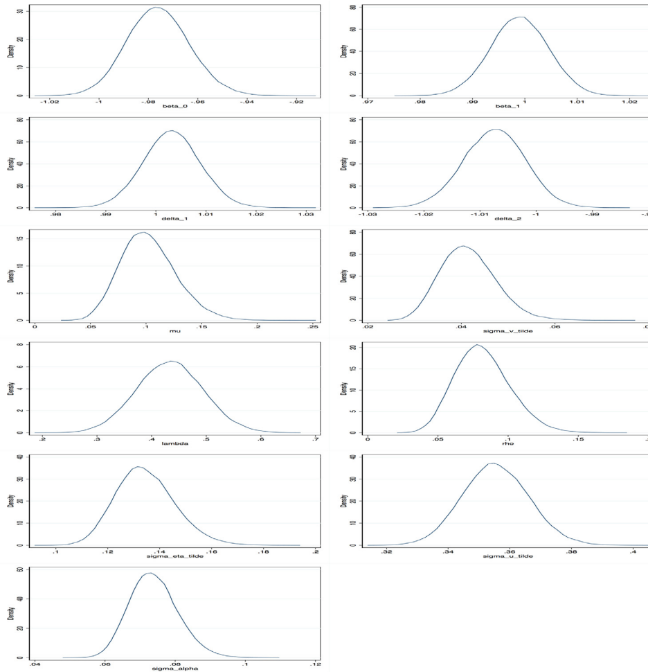
Fig. 1. Posterior distributions of parameters from the simulated data.
