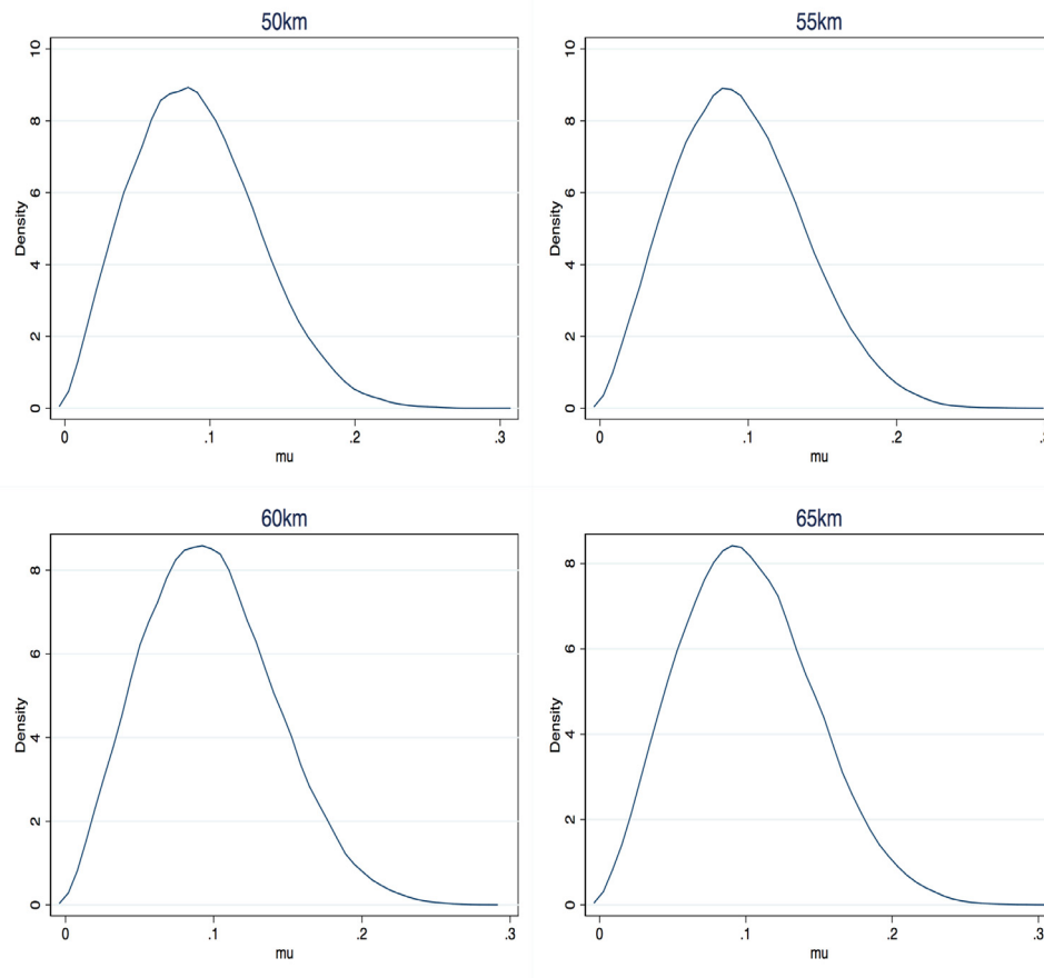
Fig. A1. Posterior distributions of \mu for the different cut-off points.
