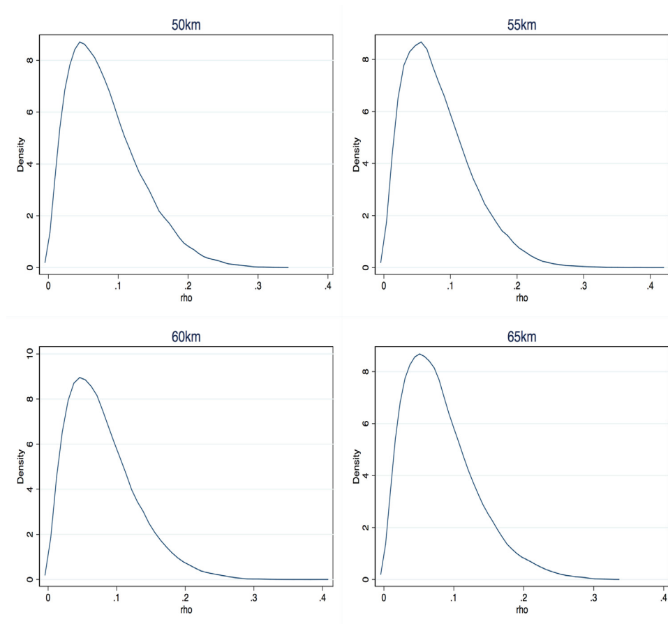
Fig. A3. Posterior distributions of \rho for the different cut-off points.
