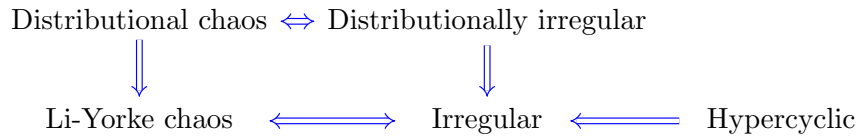
FIGURE 6. Relations between dynamical properties introduced in Section 4.
