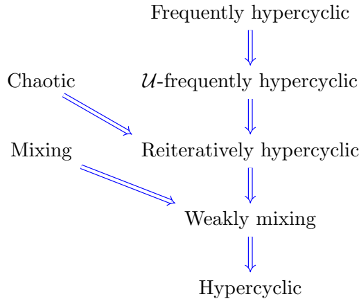
FIGURE 5. Relations between various linear dynamical properties.
