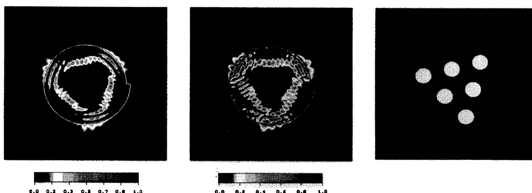
Figure 1: (a) Field intensity plot of quasiscarred resonance in the passive cavity for n = 2 and nkR \approx (29.9, -0.12) . (b) Field intensity plot of lasing pattern using Schrödinger-Bloch model for n = 2 and Re[nkR] = 30 . In figures (a) and (b), the field intensity is normalized by scaling the maximum intensity as 1. (c) Geometrical shape of selected external pumping region (white circles).
