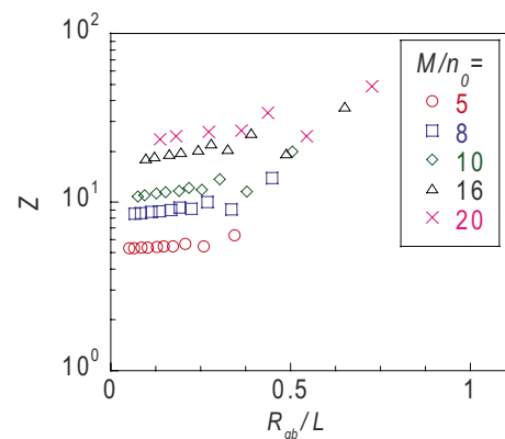
FIG. 8. (Color online) Plots of the mean number of entanglement Z per single chain as a function of L . Z gradually increases as L decreases.
