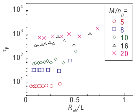
FIG. 6. (Color online) Plots of relaxation time \tau_{\mathbf{P}} of the end-to-end vector as a function of L . \tau_{\mathbf{P}} gradually increases as L decreases.
