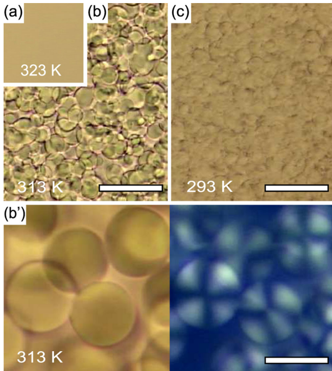
FIG. 1 (color online). Optical microscopic images obtained from the sample of \phi_{3MP} = 0.09 : (a) T = 323 K (disordered), (b) T = 313 K (onion), and (c) T = 293 K (onion). Scale bars in (b) and (c) are 100 μm. (b') A magnified view of (b) (left) and a birefringent image of the same region (right) with the scale bar being 20 μm.
