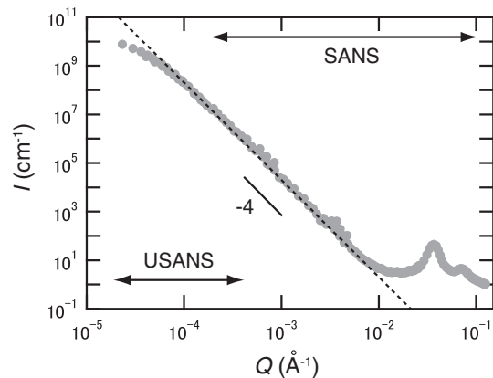
FIG. 4. Connected USANS profile obtained at PNO and SANS-J over a wide range of Q at T = 298 K and \phi_{3MP} = 0.09 . The Porod tail \propto Q^{-4} from onion surfaces can be observed in the range 1 \times 10^{-4} < Q < 5 \times 10^{-3} Å -1 .
