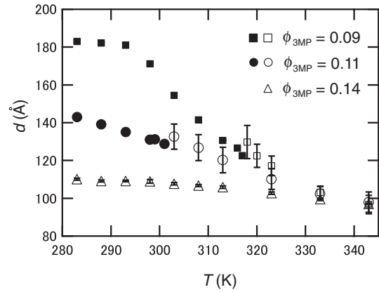
FIG. 3. Repeat distance d vs temperature T for \phi_{3MP} = 0.14 (triangle), 0.11 (circle), and 0.09 (square). Open symbols indicate data of the disordered phase while filled symbols indicate data of the onion phase. No onion appears for \phi_{3MP} = 0.14 .
