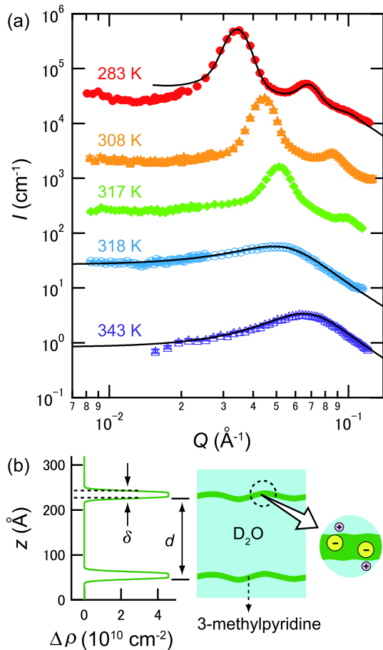
FIG. 2 (color online). (a) Temperature dependence of SANS intensity from a sample of \phi_{3MP} = 0.09 . The first-order transition occurs slightly below T = 318 K. The data at lower temperatures are shifted by multiplying 10 for better visualization. (b) Scattering density distribution at T = 283 K estimated from the formula in Ref. [20] (left) and schematic picture of the distribution of the ingredients (right). The vertical axis indicates the distance normal to the layers.
