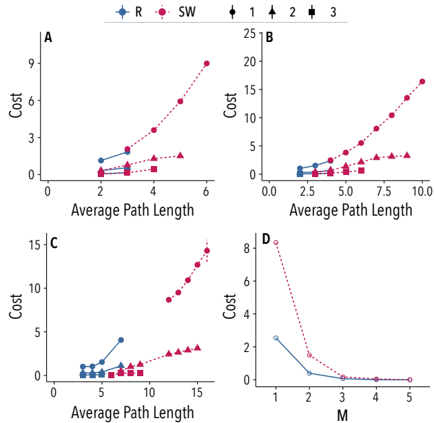
Figure 6.7: Numerical results of the model. A,B,C: Average final cost (in 10^4 ) of the cheapest path after a period of 10^4 rounds as a function of the average path length of the network. Different panels correspond to different network sizes: 26 ( A ), 50 ( B ), and 1000 ( C ) nodes; colours correspond to different network models: random (blue) and small-world (magenta); and different shapes correspond to different values of the number M of disjoint paths. For each configuration, there were generated 10000 networks of size 26, 50, and 1000, according to the Watts-Strogatz algorithm [59] with p = 0.1, 1 and average degree from 2 to 10. The initial cost was set to 0 and the increment/decrement ratio was fixed to the experimental value ( \sigma/\rho = 2.4 ). Results for M > 5 are not shown as costs converge fast to 0. D: Mean value of the cost of the cheapest path versus M for the same networks.
