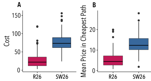
Figure 6.2: Network topology affects trading costs and prices. A: Cost of the cheapest path for the random network of 26 nodes (R26), and for the small-world network of 26 nodes (SW26). B: Mean price of participants in cheapest path for the same networks. Lines in the boxes denote the medians, whereas boxes extend to the lower- and upper-quartile values. Whiskers extend to the most extreme values within 1.5 interquartile range (IQR).
