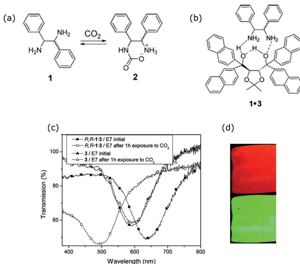
Figure 18. a) Chiral dopant containing diamine groups ( 1 ) that transforms into a carbamate ( 2 ) upon CO 2 exposure. b) Complex chiral dopant 1.3 (produced via mixing 3 , a TADDOL derivative, with 1 ) used by Han et al. [162] to dope E7 (LC host). c) Transmission spectra of E7 samples doped with 1.3 and 3 , before (closed symbols) and after (open symbols) exposure to CO 2 . d) Images of an E7 sample doped with 1 , before (top) and after (bottom) exposure to CO 2 for 1h. Reproduced with permission. [162] Copyright 2010, American Chemical Society.
