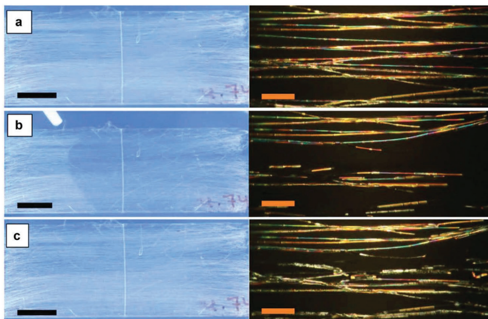
Figure 10. Aligned mat with coaxially spun PVP-5CB fibers a) before, b) during and c) after toluene exposure. Images on the left were taken when the mat was observed under nonchromatic crossed polarizers (scale bar 10 mm). In the right column, the images were captured during POM observation of the mat using crossed polarizers (scale bar 80 \mu\text{m} ). Reproduced with permission under the terms of the CC-BY-NC-ND 4.0 license. [44] Copyright 2016, The Authors, published by Taylor & Francis.
