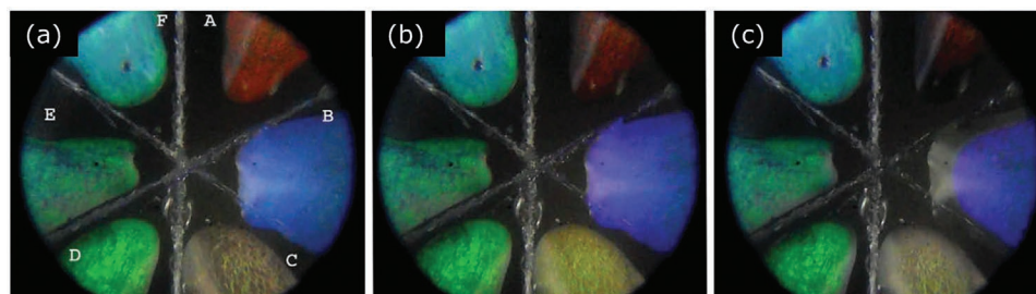
Figure 19. Color changes of six chiral liquid crystal droplets with different compositions (from A to F) as observed with polarizing optical Microscopy. a) Initial state, b) response to 5 μL of cyclohexane, c) response to 10 μL of cyclohexane. Reproduced with permission. [48] Copyright 2019, Taylor & Francis.
