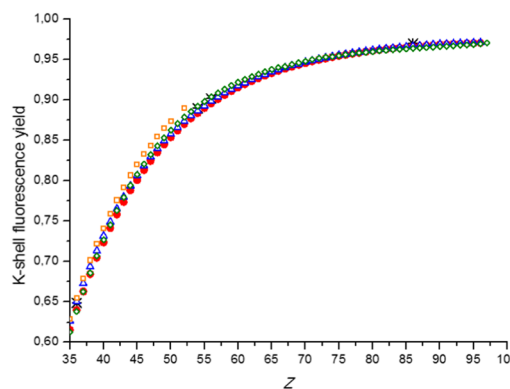
(b) Theoretical K-shell fluorescence yield values ( 35 \leq Z \leq 96 )
