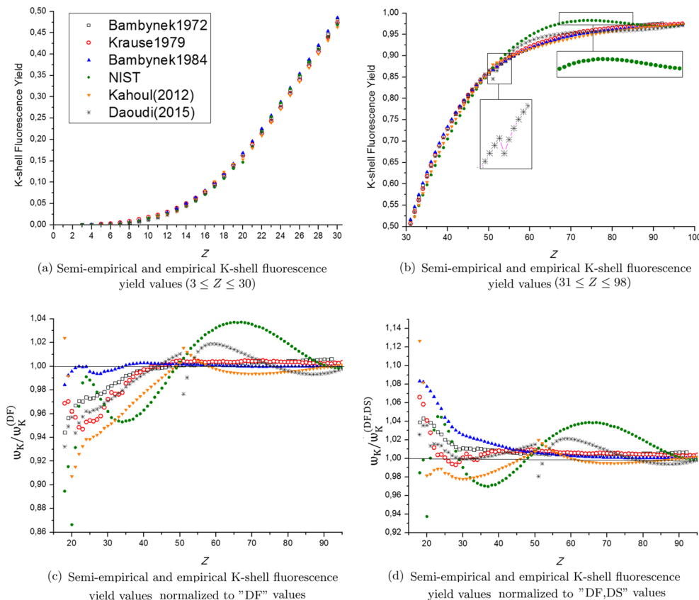
FIGURE 2 “Bambynek 1972”: Values from Bambynek et al. earlier semi-empirical fit. [22] “Krause 1979”: values from Krause’s semi-empirical fit. [40] “Bambynek 1984”: values from Bambynek et al. later semi-empirical fit. [41] “NIST”: semi-empirical fit values presented in NIST’s Fundamental Parameters Database. [28] “Kahoul”: values from Kahoul et al. empirical fit. [29] “Daoudi”: values from [Colour figure can be viewed at wileyonlinelibrary.com ]
