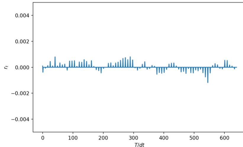
Figure 9. An Arbitrary Simulated Path for r_t
