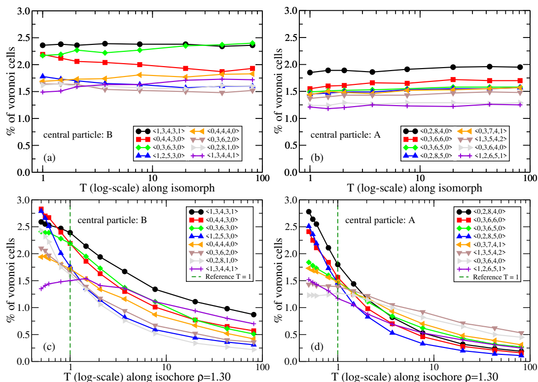
Figure 12. Temperature dependence of the occurrence of eight of the most abundant Voronoi structures at the reference state point (\rho, T) = (1.30, 1.00) , plotted for the NiY 2 binary mixture as follows: along the isomorph as a function of the logarithm of the temperature (a,b), along the \rho = 1.30 isochore as a function of the logarithm of the temperature (c,d). In (a,c) the central particle is of type B, in (b,d) it is an A particle. The Voronoi structures are isomorph invariant to a good approximation, but vary significantly along the isochore.
