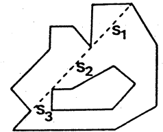
Fig. 4. A non-primitive chord s which consists of three primitive chords s_1, s_2 and s_3 .
