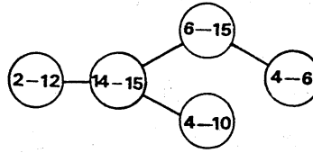
Fig. 9. Intersection graph G(P) of minimally effective chords of P.
