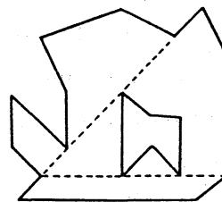
Fig. 6. Effective chords which are not primitive.
