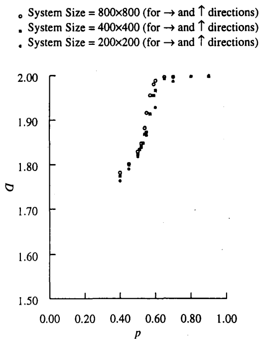
Figure 2: Fractal dimension by box counting
