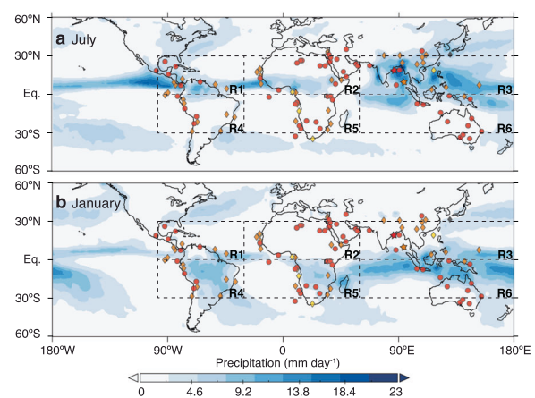
Fig. 1 Present-day tropical precipitation. Map showing mean (1981–2010) CMAP global precipitation 121 rates during July (a) and January (b), conveying seasonal ITCZ migration and monsoonal development. Gridded boxes highlight tropical division of Regions 1 through to 6. Orange diamonds represent proxy records used for both time series and anomaly-map comparisons (Figs. 2 and 3), yellow diamonds represent proxy records used only for time series (Fig. 2), red circles represent proxy records used only in the anomaly map (Fig. 3) and stars represent proxy records generated in this study (red, U1446 and orange, U1448) (see Methods and Supplementary Data 1 for detail and references). Precipitation data available from https://psl.noaa.gov/data/gridded/data.cmap.html . Map produced using Panoply (source: https://www.giss.nasa.gov/tools/panoply/ ).
