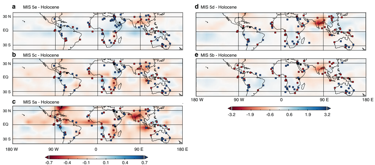
Fig. 3 MIS 5 hydroclimate reconstructions compared with the Holocene. Emulated anomaly maps of MIS 5 time slices with respect to the Holocene (12–0 ka) a MIS 5e—Holocene, b MIS 5c—Holocene, c MIS 5a—Holocene, d MIS 5d—Holocene, e MIS 5b—Holocene. Proxy data are superimposed; blue square = “wetter” than Holocene average, red square = “drier” than Holocene average and black square = no change (Methods and Supplementary Data 1). Emulated data are integrated from native model resolution (64 × 32 grid cells) onto 32 × 16 resolution, to smooth out grid-scale variability. Maps were produced using Panoply (source: https://www.giss.nasa.gov/tools/panoply/ ).
