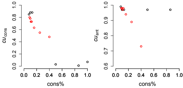
Figure 10: Left: Plot of \text{cons}\% to cu_{\text{cons}}\% . Right: Plot of \text{cons}\% to cu_{\text{ant}}\% . Red dots represent runs using \sigma_{IRC} .
