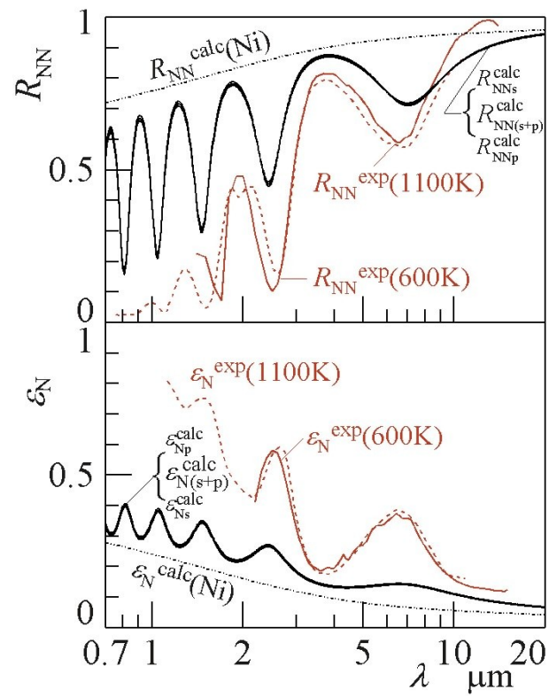
Figure 5 Spectra of reflectance R_{NN} and emittance \varepsilon_N of the film system (measured and calculated)
