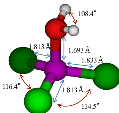
Figure 3: The structure of the stable reactant complex (RC), Cl 3 B—OH 2 .
