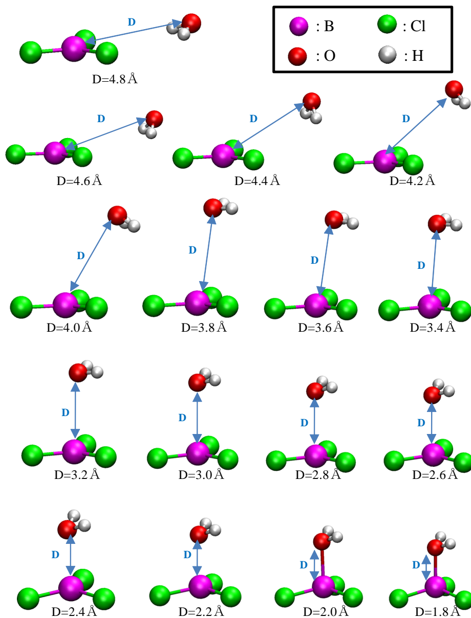
Figure 1: Optimized configurations of BCl 3 and H 2 O at the given B—O distance ( D ).
