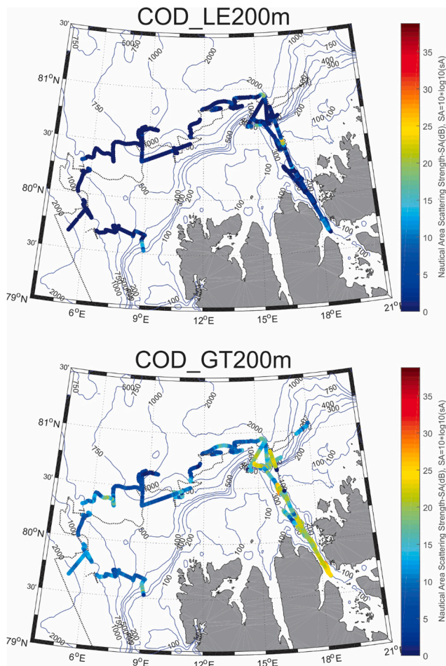
Fig. 9. Acoustic registrations per 1 nmi scrutinized as Atlantic cod along cruise tracks during September 2016 with RV Helmer Hanssen west and north of Svalbard. Upper panel: Integrated values of NASC ( \text{m}^2 \cdot \text{nmi}^{-2} ) at 38 kHz between \sim 15 and 200 m depth. Lower panel: Integrated values of NASC ( \text{m}^2 \cdot \text{nmi}^{-2} ) at 38 kHz between 200 m and bottom. Data presented as nautical area scattering strength [ S_A , dB re 1 \text{ m}^2 \cdot \text{nmi}^{-2} ], S_A = 10 \log_{10}(s_A) . Black stippled lines represent along-track locations where integrated NASCs for the given category were originally 0.0. However, a small value of 0.0001 was added to all data in the linear domain so that log-transformation and visualization could be undertaken.
