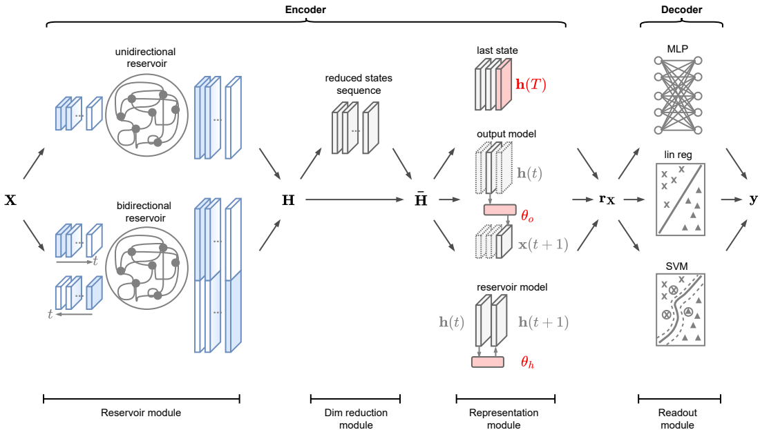
Fig. 2: Framework overview. The encoder generates a representation r_X of the MTS X , while the decoder predicts the label y . Several models are obtained by selecting one variant for each module. Arrows indicate mutually exclusive choices
