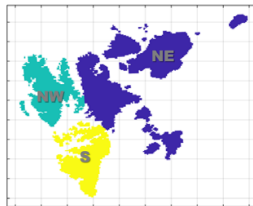
Figure 6.6.4: Svalbard regions used in Table 6.6.1.
