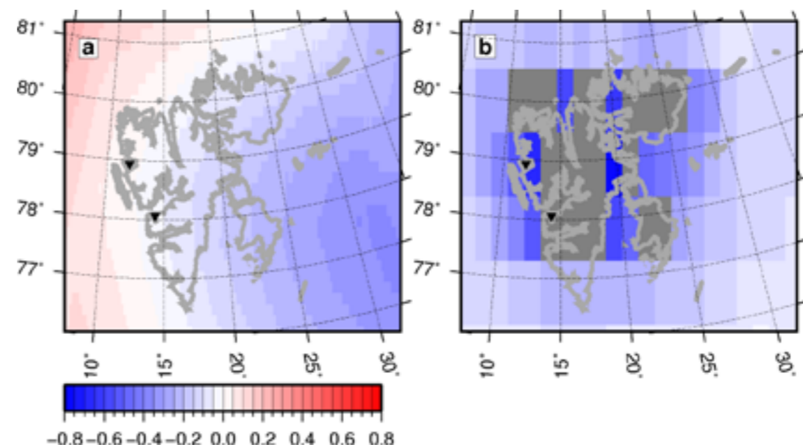
Figure 8.4.3. Relative sea-level change (m) due to GIA (panel a) and future glacier changes for RCP4.5 (panel b) over the period 1986–2005 to 2081–2100. Results are from IPCC AR5 and both show the mean field.
