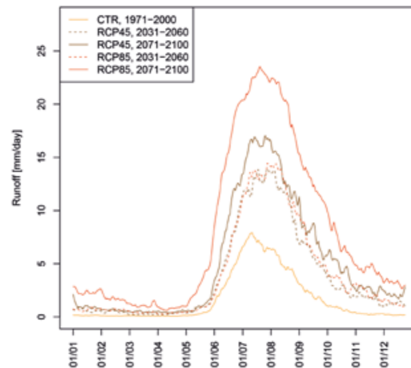
Seasonal runoff distribution, all of Svalbard
