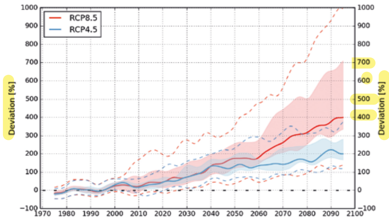
Mean annual runoff - Svalbard
