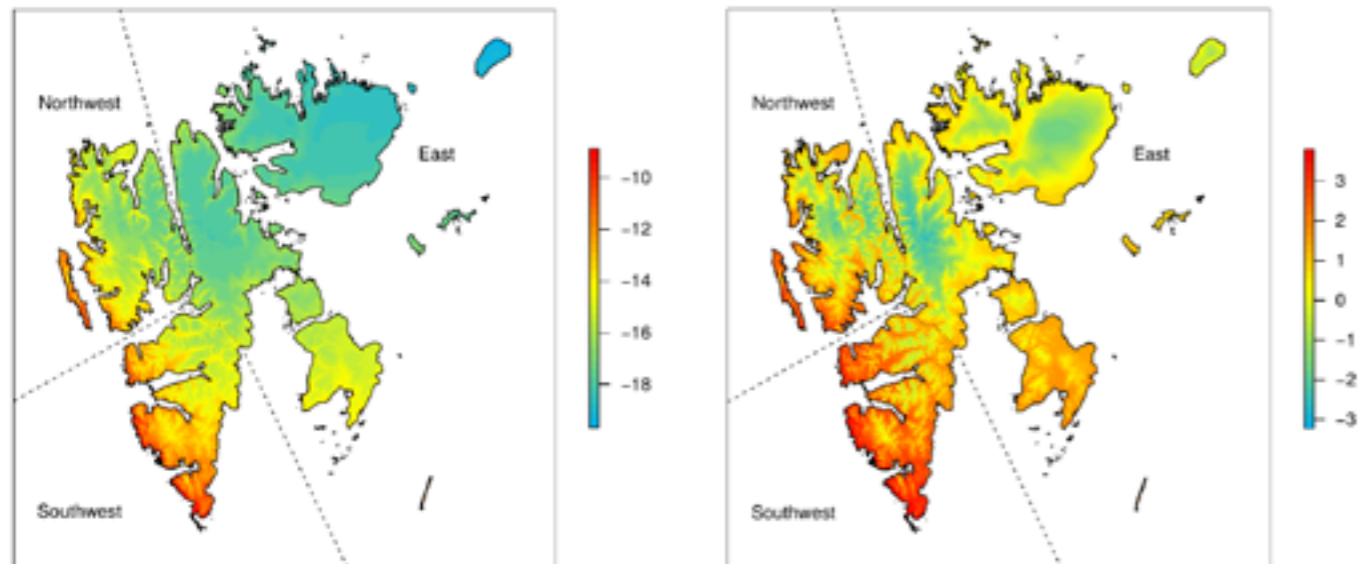
Figure 4.1.2. Winter (Dec-Jan-Feb; left) and summer (Jun-Jul-Aug; right) temperature [°C] averaged over 1971-2000 based upon the Sval-Imp dataset. Note that the colour scales are different!
