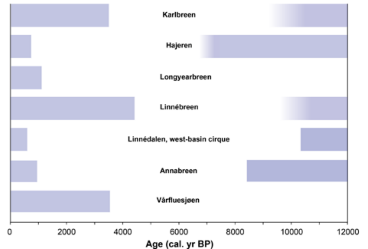
Figure 6.1.1. A compilation of Holocene glacier reconstructions from Svalbard, modified after De Wet et al. (2017). Blue fields indicate prolonged periods of glacier activity. Included records derive from (north) west Spitsbergen: Karlbreen and Hajeren from the Mitra peninsula (79°N, 11°E) (Røthe et al., 2015; van der Bilt et al., 2015), Longyearbreen (78°N, 15°E) (Humlum et al., 2005), Linnébreen and the west-basin cirque in Linnédalen (78°N, 14°E), Annabreen on Amsterdamøya (79°N, 11°E) (De Wet et al., 2017), and Vårfluesjøen (79°N, 15°E) (Røthe et al., 2018).
