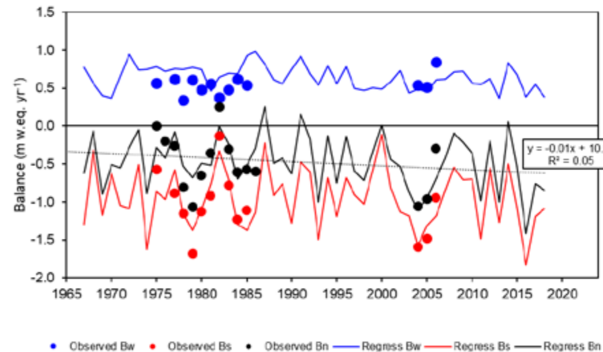
Figure 10.2.7 Winter, summer and net balance for Bogerbreen, near Longearbyen. Blue lines show the total accumulation on the glacier during the winter, converted to an area average thickness of water (metres of water equivalent, m w.eq.); red lines similarly show the net melt over the summer, while black lines are the sum of the two, or the total mass gained or lost through the glacier surface processes over the year. The observations (symbols) are extended by performing a linear fit of the Bogerbreen to the long-term Austre Brøggerbreen record. The trend is shown for the regressed net balance.
