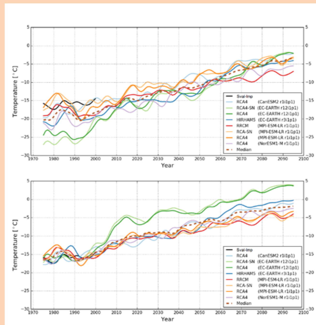
Figure B5.1 The Arctic CORDEX and CCLM projections of winter (DJF) temperatures for Svalbard under emission scenario RCP8.5. The solid black line shows results for the Sval-Imp. The dashed brown line indicates the median of the Arctic CORDEX ensemble. Upper panel: original Arctic CORDEX results. Lower panel: bias-adjusted Arctic CORDEX results.
