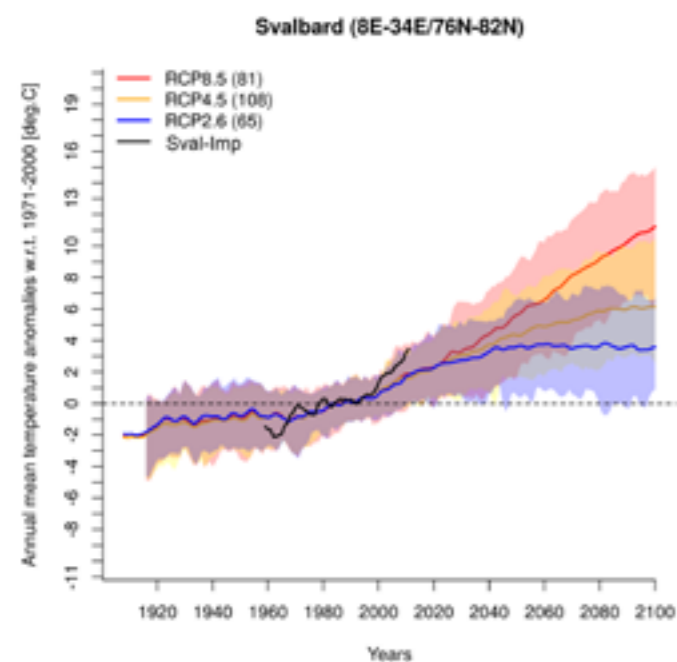
Figure 4.1.4. Annual mean temperature anomalies [°C] as simulated by the CMIP5 global climate model runs (without downscaling) following RCP2.6 (blue), RCP4.5 (orange) and RCP8.5 (red) emission scenarios. The envelopes are based on the 5th and 95th percentiles of the multi-model simulations, hence, display the 90 % spread over the number of runs (indicated in the legend between parentheses) used for each ensemble simulations. The black line shows the Sval-Imp dataset, which is applied as reference dataset. All the simulations have been subject to a spline smoother to extract the inter-annual climate change signal.
