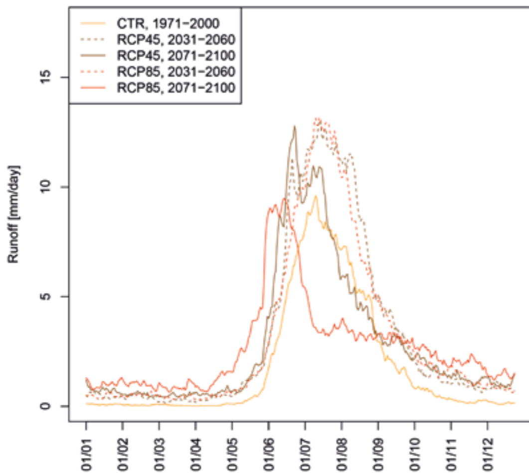
Seasonal runoff distribution, Longyearelva
