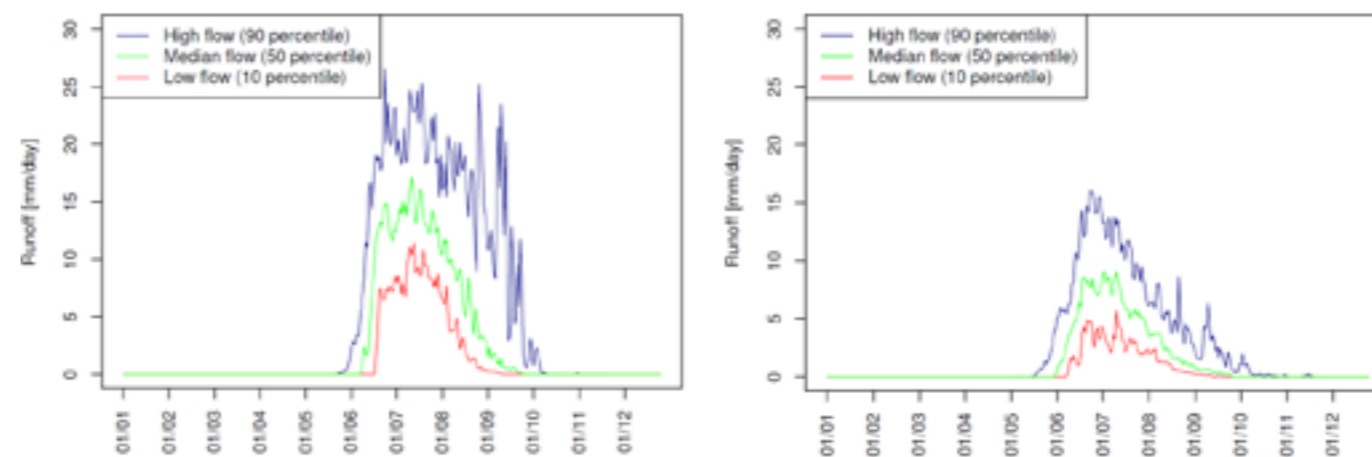
Figure 5.1.1 Seasonal cycle at Bayelva (1989–2017) and De Geerdalen (1991–2015).
