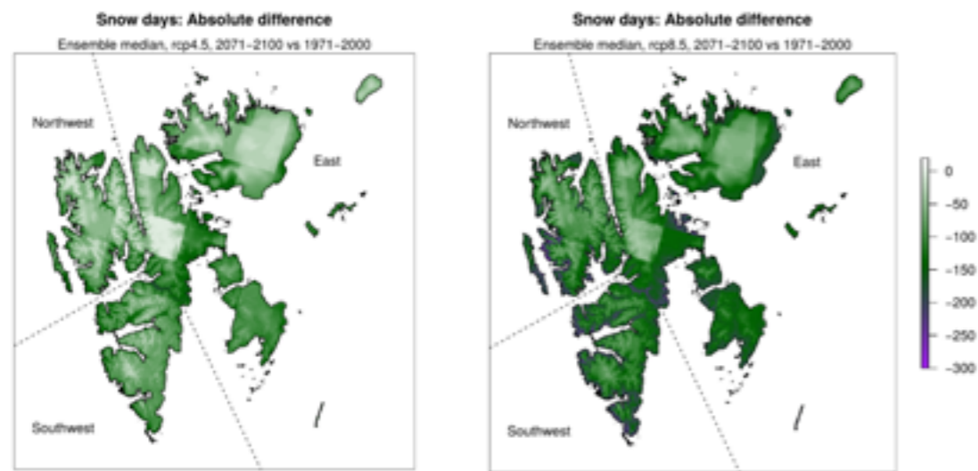
Figure 5.2.6. Changes in snow season duration (annual number of snow days) from 1971–2000 to 2071–2100, for RCP4.5 (left) and RCP8.5 (right). Simulations show the ensemble median for the bias-adjusted Arctic CORDEX runs (1 km spatial resolution).
