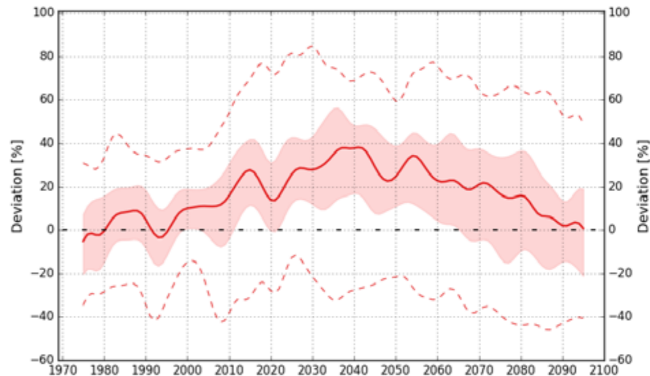
Mean annual flood - Longyearelva
