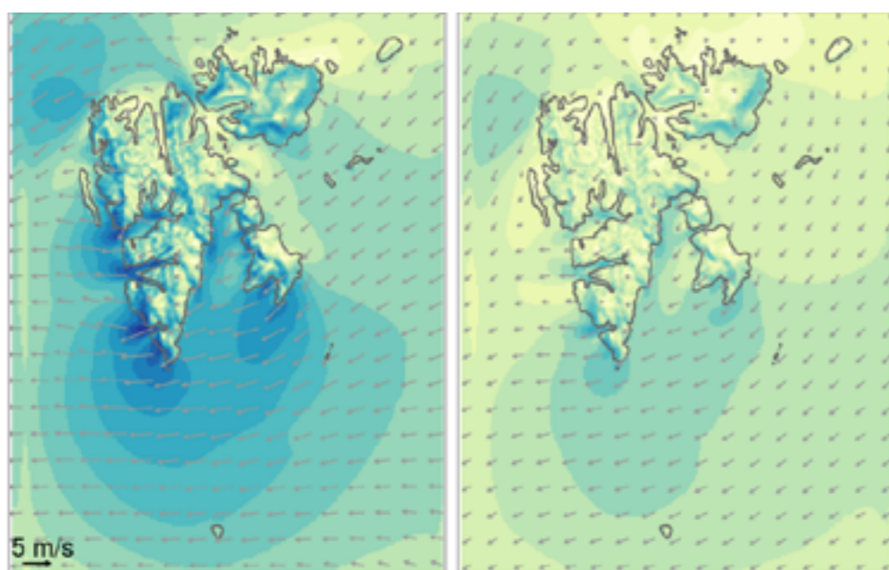
Figure 4.5.1 Simulated average wind speed and direction in winter (November-April) and summer (May-October) for the reference period 1971-2000, based on the CCLM 2.5 km model.
