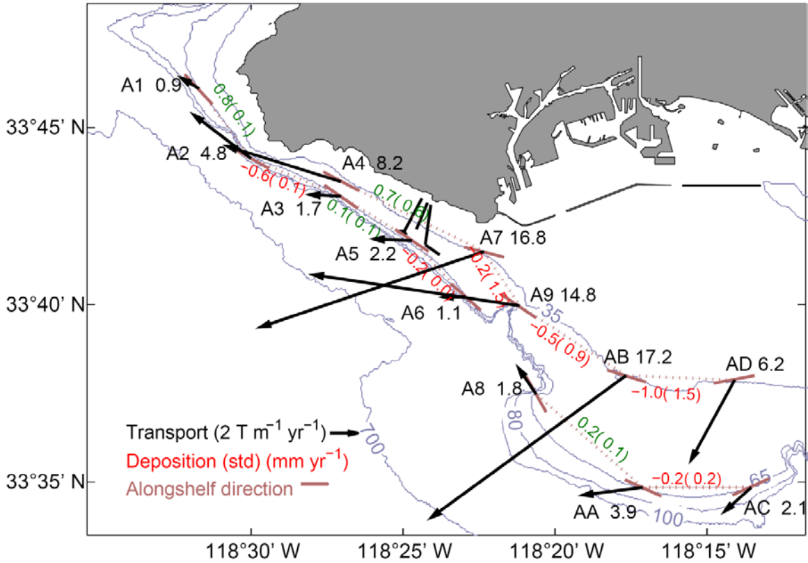
Figure 12. Annual average horizontal sediment-transport rates computed by the 1DV model at LACSD ADCP sites. The magnitude of flux is noted in black at each station location. Shown in red and green is the mean difference in alongshore component of transport between adjacent sites along dotted lines, converted to erosion rates (negative, red) or deposition rates (positive, green) with uncertainty from jackknife estimates in parentheses. The alongshore direction at each site is shown in brown.
