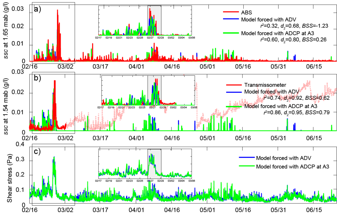
Figure 4. Model evaluation at Site B3 (a) Calculated (blue with ADV input at 1.41 mab, green with ADCP input at A3 at 3 mab) and measured (red) ssc at 1.65 mab by the ABS. Skill scores are for period of resuspension event highlighted in gray in the zoom box after filtering both measurements and model output with a 4-hour low-pass filter. (b) Calculated (blue with ADV input at 1.41 mab, green with ADCP input at A3 at 3 mab) and measured (red) suspended-sediment concentration ssc at 1.54 mab by the transmissometer. Dotted red line shows obvious corrupted data that we did not take into account in our calculations. Skill scores are for period of resuspension event highlighted in gray in the zoom box after the same filtering as previous. (c) Bottom shear stress calculated by the model with ADV input (blue) and ADCP at A3 (green) during the same period as previous, from February to June 2004.
