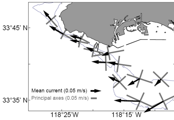
Figure 9. Mean current velocity and principal axes of variation for LACSD ADCP measurements in the bottom bin (3 mab) for the entire record (Fig. 8 and Table 3).
