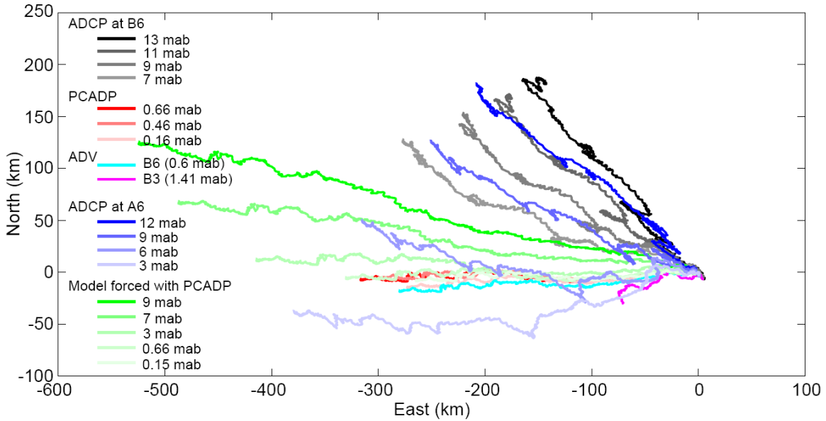
Figure 7. Progressive vectors for measured and modeled flow, February to June 2004 at USGS Site B6 and nearby LACSD Site A6. Black and gray lines are progressive vectors measured between 7 and 13 mab by the USGS ADCP at B6. Red and pink lines represent measurements between 0.16 and 0.6 mab by the USGS PCADP on the same tripod. Cyan lines represent measurements by the USGS ADV at 0.6 mab on the same tripod. Blue and light blue lines represent measurements from the LACSD ADCP at site A6, located approximately 1.7 km SSE from B6. Green lines represent modeled flow at various elevations, forced by PCADP measurements at 0.16 mab.
