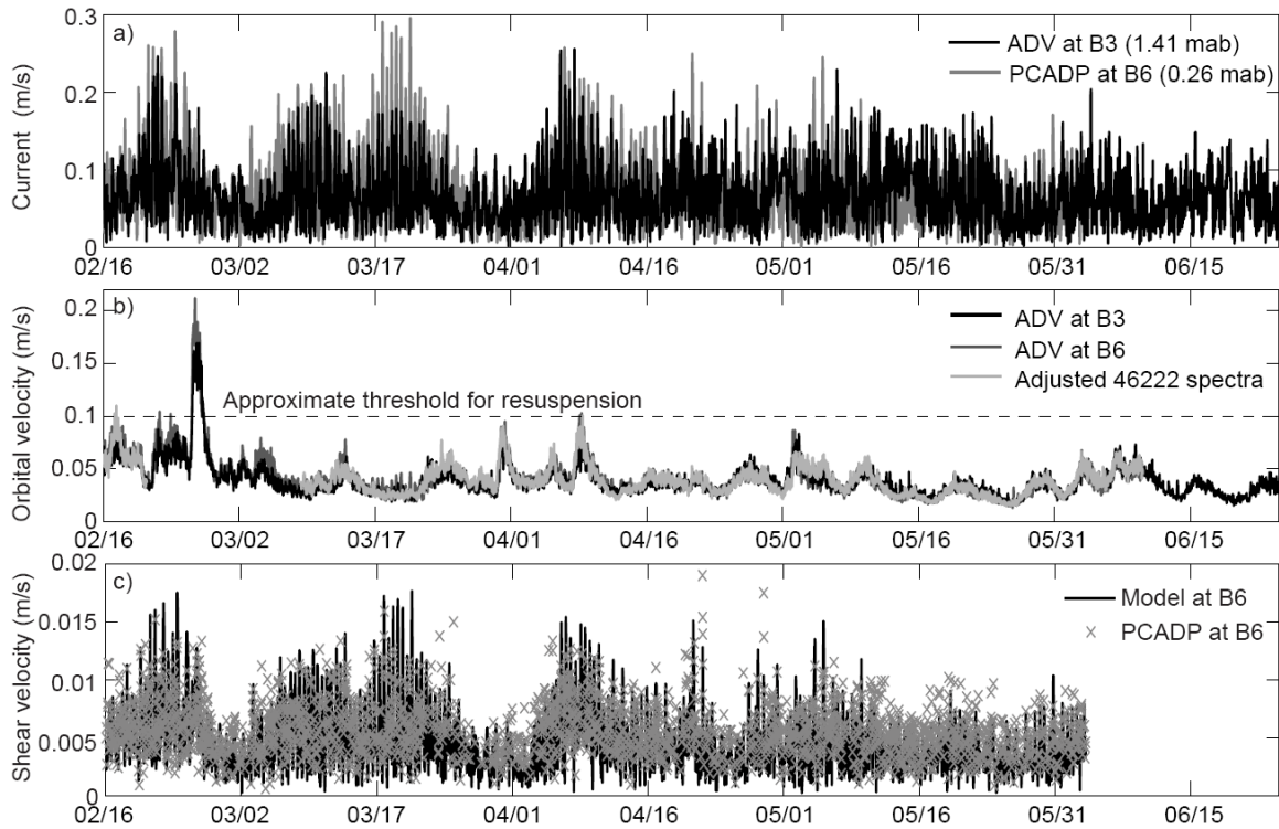
Figure 3. Data and model results at sites B3 and B6. (a) Current speed at 1.41 mab measured by the ADV and used to force the model at B3 (black) and current speed at 0.26 mab measured by the PCADP and used to force the model at B6 (gray). (b) Wave-orbital velocity calculated directly from the ADV measurements at B3 (black) and B6 (dark gray), and from CDIP buoy 46222, adjusted for refraction and shoaling (light gray). The dotted line at 0.1 \text{ m s}^{-1} indicates the approximate threshold for resuspension of PV sediment (Wiberg et al., 2002; see text). (c) Bottom shear velocity estimated from log fits to measured PCADP profiles (only those with r^2 > 0.98 ; xs) and calculated by the model (line).
