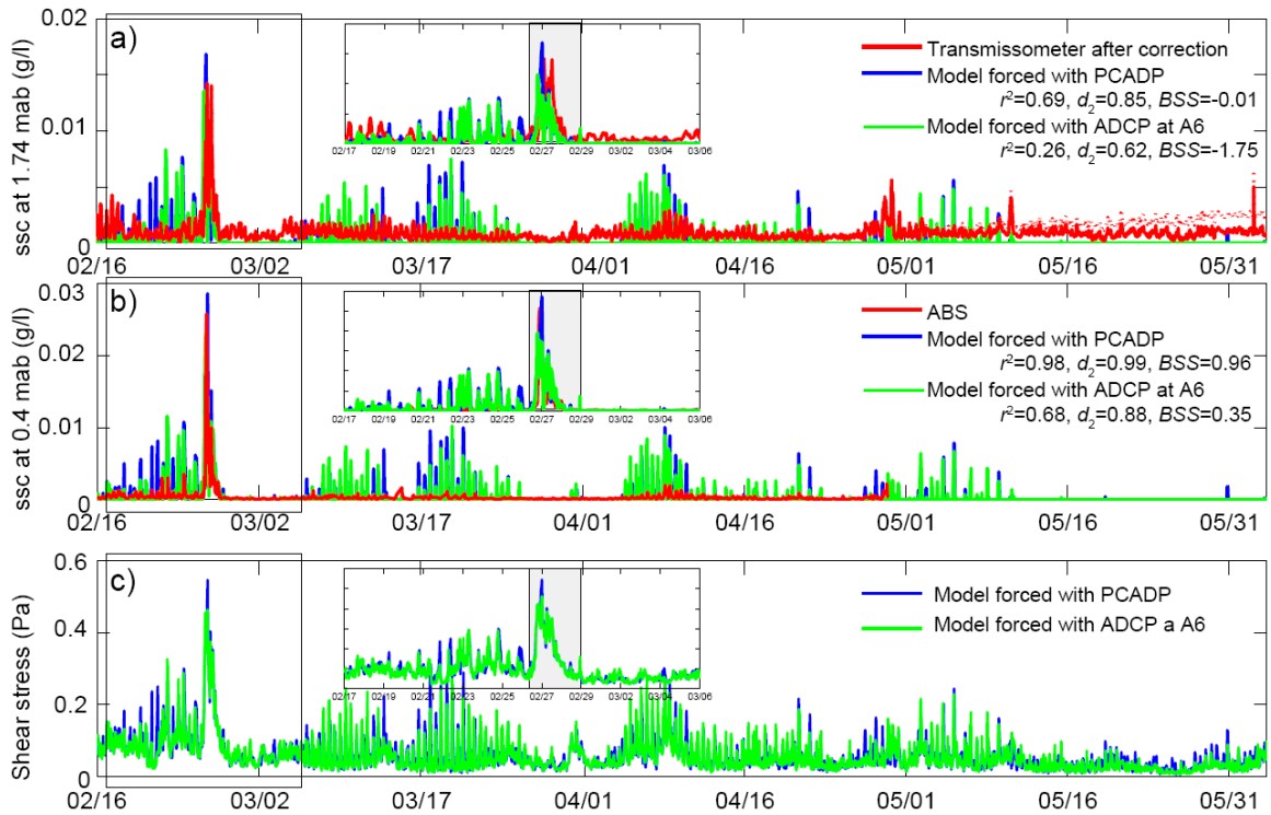
Figure 5. Model evaluation at Site B6. (a) Calculated (blue with PCADP input at 0.26 mab, green with ADCP at A6 at 3 mab) and measured (red) suspended-sediment concentration ssc at 1.74 mab by the transmissometer. Dotted red line shows ssc measured by the transmissometer before correction for biofouling. Skill scores are for period of resuspension event highlighted in gray in the zoom box after filtering both measurements and model output with a 4-hour low-pass filter. (b) Calculated (blue with PCADP input at 0.26 mab, green with ADCP at A5 at 3 mab) and measured (red) ssc at 0.40 mab by the ABS. Skill scores are for period of resuspension event highlighted in gray in the zoom box after filtering. (c) Bottom shear stress calculated by the model with PCADP input (blue) and ADCP at A6 (green) during the same period as previous, from February to June 2004 at site B6.
