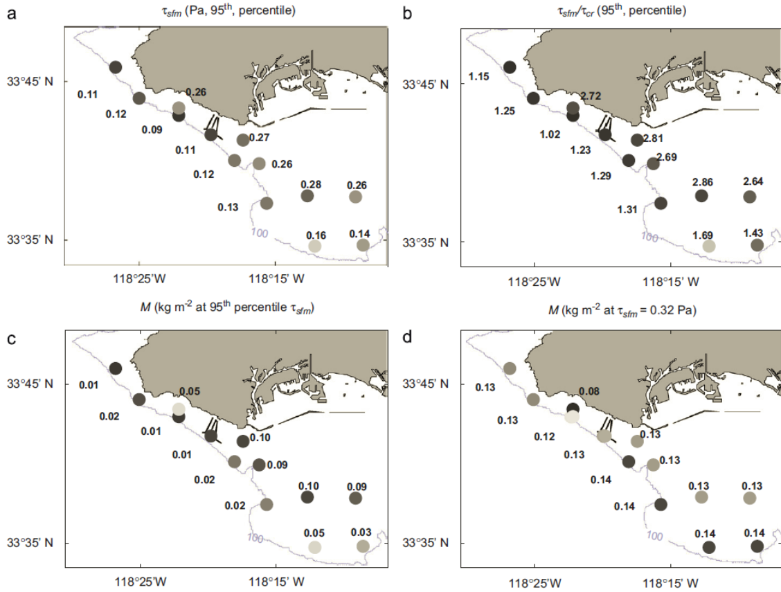
Figure 11. Comparison of bottom stress and bed mobility from model calculations. a) Bottom shear stress (95 th percentile of cumulative distribution). b) ratio of bottom shear stress to critical shear stress (non-dimensional; 95 th percentile of cumulative distribution). c) Amount of material eroded M , computed from local erosion-chamber results and using the 95 th percentile of bottom stress. d) Amount of material eroded at bottom stress of 0.32 Pa. Only the 100-m contour is shown.
