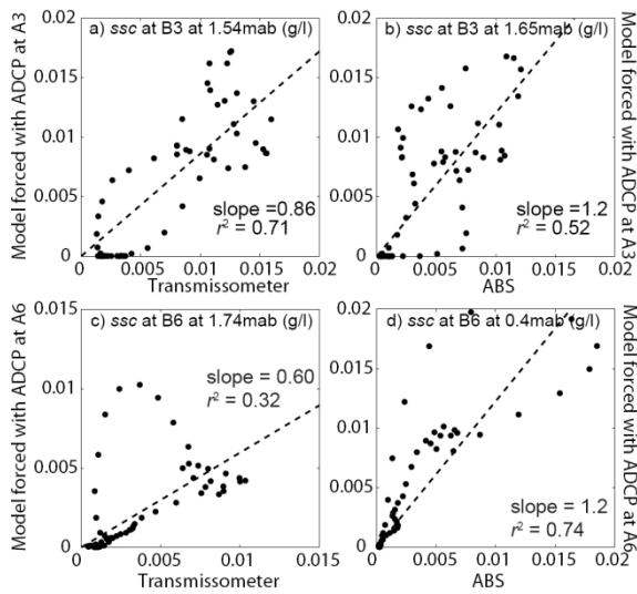
Figure 6. Correlations forced through zero between observed data and model results after filtering both with a 4-hour low-pass filter. (a) at B3, between transmissometer at 1.54 mab and the model forced with ADCP data at A3. (b) at B3, between ABS at 1.65 mab and the model forced with ADCP data at A3. (c) at B6, between transmissometer at 1.74 mab and model forced with ADCP data at A6. (d) at B6, between ABS at 0.4 mab and model forced with ADCP data at A6. Dashed line in each subplot is the linear regression forced through zero. The slope and correlation coefficient squared are indicated.
