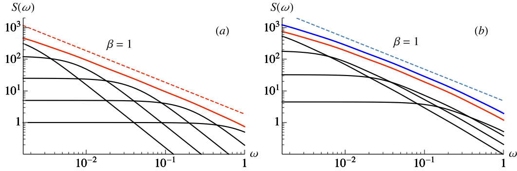
FIG. 1. (a) The solid red line shows the sum S^{(0)}(\omega) in Eq. (16), with N = 5, \beta = 1, \tau_1 = 1, b_1 = 1 , and a = 5 . The dashed red line shows a power law of 1/f^\beta , with \beta = 1 . The black lines show the contribution from each term in the aggregation. (b) The red line shows the sum S^{(cr)}(\omega) , while the blue line shows S^{(0)}(\omega) + S^{(cr)}(\omega) . The dashed blue line shows the power-law spectrum we approximate, given the same forcing for all modes. The black lines show the contribution to S^{(cr)}(\omega) for each k : \sum_{j < k} 2b_k b_j (\omega_k \omega_j + \omega^2) [(\omega_j^2 + \omega^2)(\omega_k^2 + \omega^2)]^{-1} .
