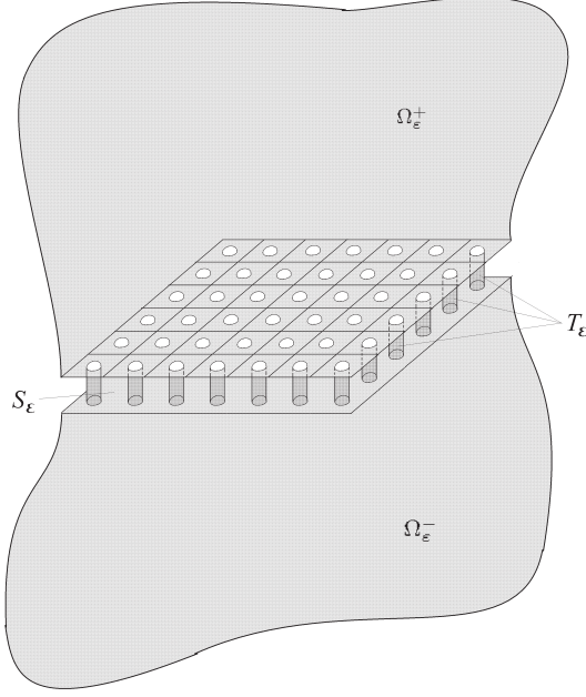
Figure 2: The domain \Omega_\varepsilon
