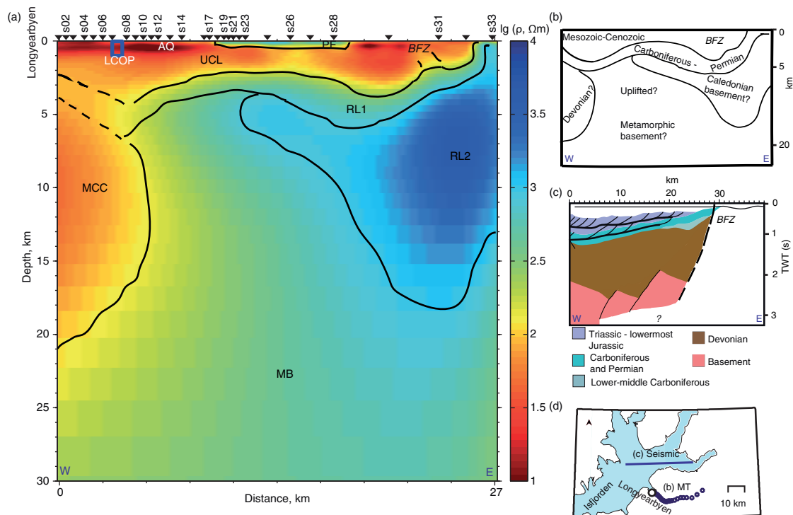
Fig. 3 (a) The final two-dimensional (2D) magnetotelluric (MT) model. The colour scale ( \lg ) is shown in \lg_{10} . An error floor of 5% is assigned on the inverted data, and the inversion is started from a 100\text{-}\Omega\text{m} half-space model. The data misfit of the final model is shown in Fig. 4. (b) Geological interpretation of the MT model. (c) A schematic geological cross-section derived from a seismic section (parallel to the MT profile) in eastern Isfjorden, redrawn from Blinova et al. (2012). The y axis is given in two-way-travel time (TWT, s), where each second represents two-way-travel time (see Blinova et al. 2012). (d) The offshore seismic transect and the measured MT sites are shown in the same map to illustrate the position of the two profiles in relation to each other. Isfjorden is indicated to facilitate comparison with Fig. 1. The MT result is comparable to interpretations derived from seismic sections as in (c) and to the stratigraphic section marked by the rectangle in Fig. 1b. Geological and other features are abbreviated as follows: Longyearbyen CO 2 Lab's well park (LCOP); permafrost (PF); upper-crust conductive layer (UCL); mid-crust conductor (MCC); resistive layer 1 (RL1); resistive layer 2 (RL2); metamorphic basement (MB).
